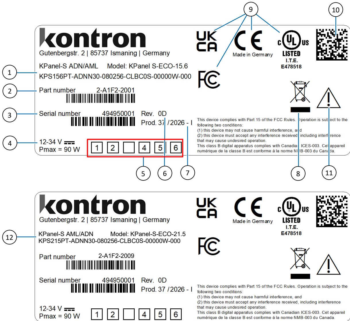
Figure 2: Type Label Example (KPanel S-AML/ADN-15.6 & KPanel S-AML/ADN-21.5)
