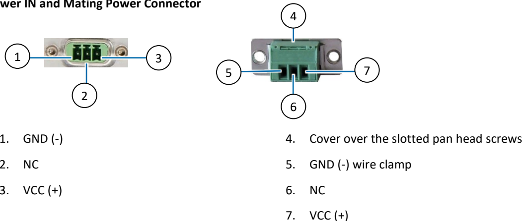
Figure 18: Power IN and Mating Power Connector
