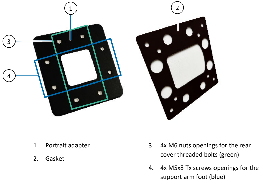
Figure 14: Portrait Adapter and Gasket
