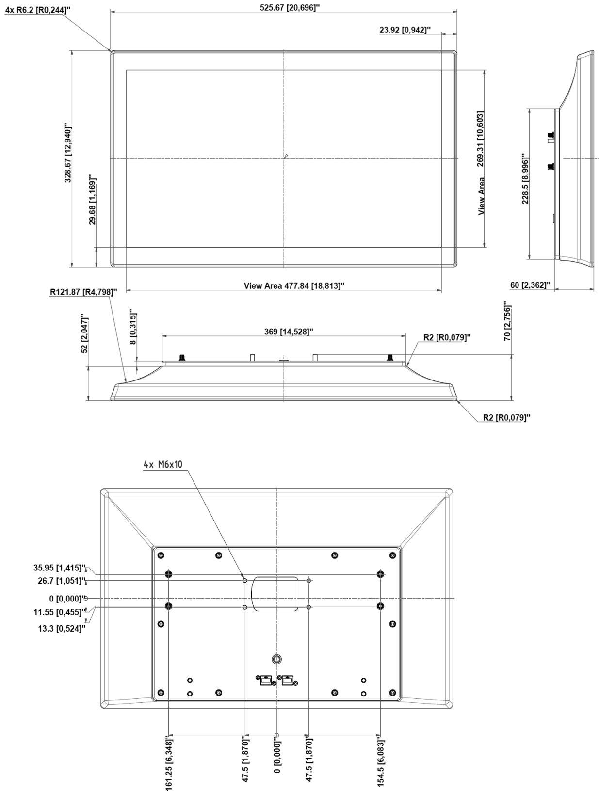
Figure 12: 21.5" Dimension Diagram (mm/inch)
