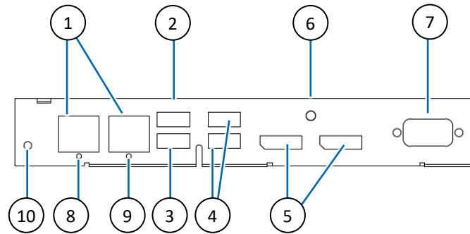
Figure 7: Interface Panel – KPanel S-AML/ADN
