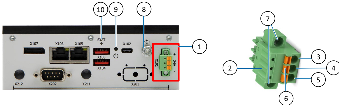
Figure 20: 24 VDC Power IN Connector and Mating Power Connector
