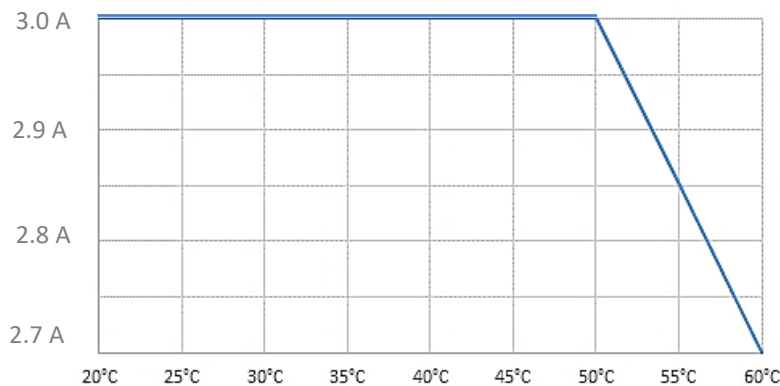
Figure 17: Derating Current USB-C Port (X102) versus Temperature Curve
