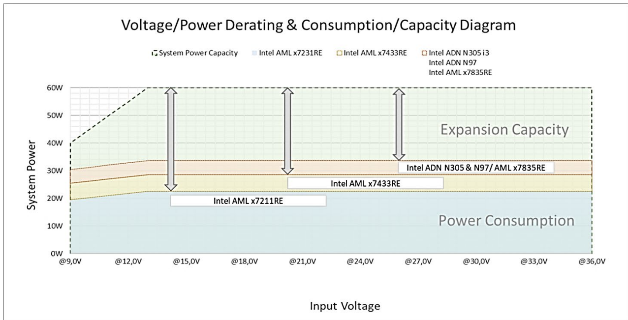
Figure 24: Voltage/Power Derating and Consumption/Capacity Curves
