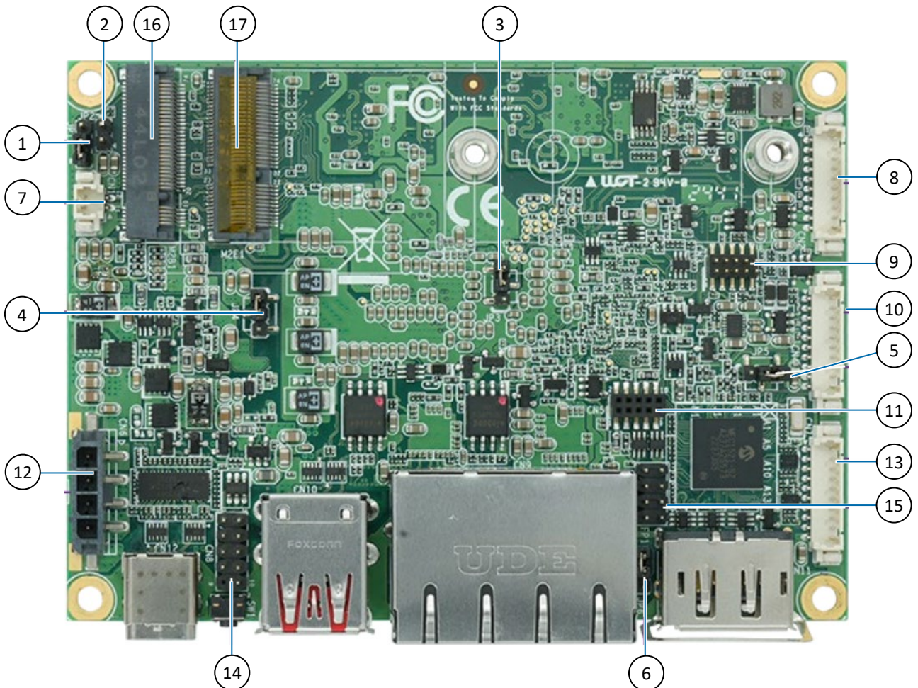
Figure 10: 2.5"-SBC-AML/ADN Onboard Components- Top Side
