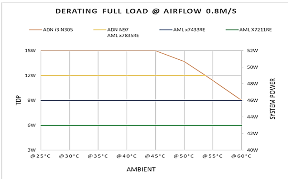
Figure 15: Derating TDP verses Temperature Curves (with full load & airflow 0.8 m/s)
