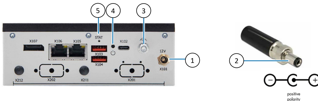
Figure 21: Power IN 12 VDC Connector and Mating Power Connector
