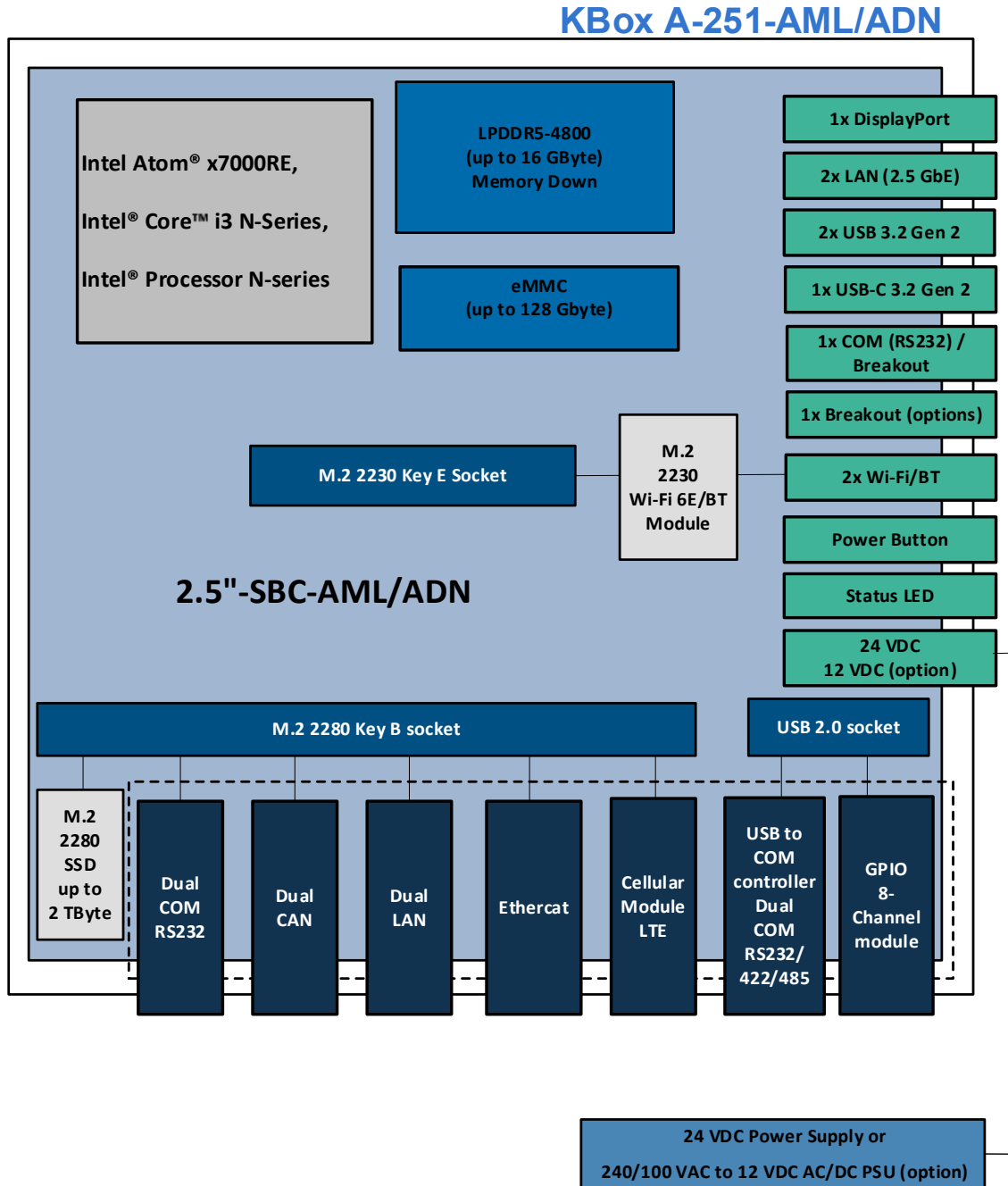
Figure 23: Block Diagram KBox A-251-AML/ADN
