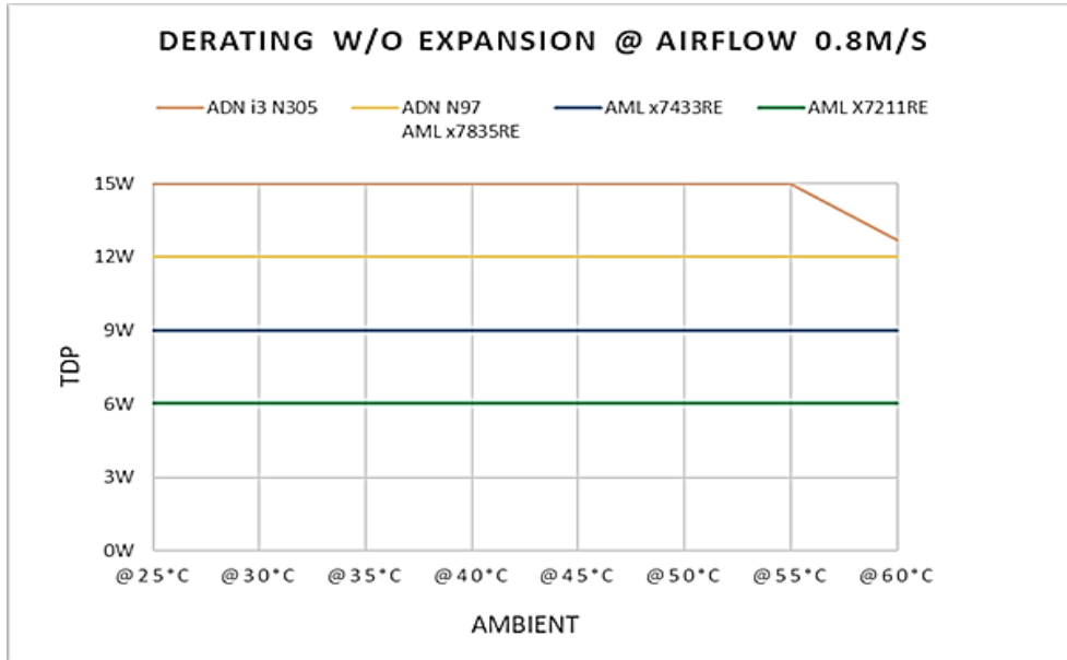
Figure 14: Derating TDP verses Temperature Curves (without expansion & airflow 0.8 m/s)
