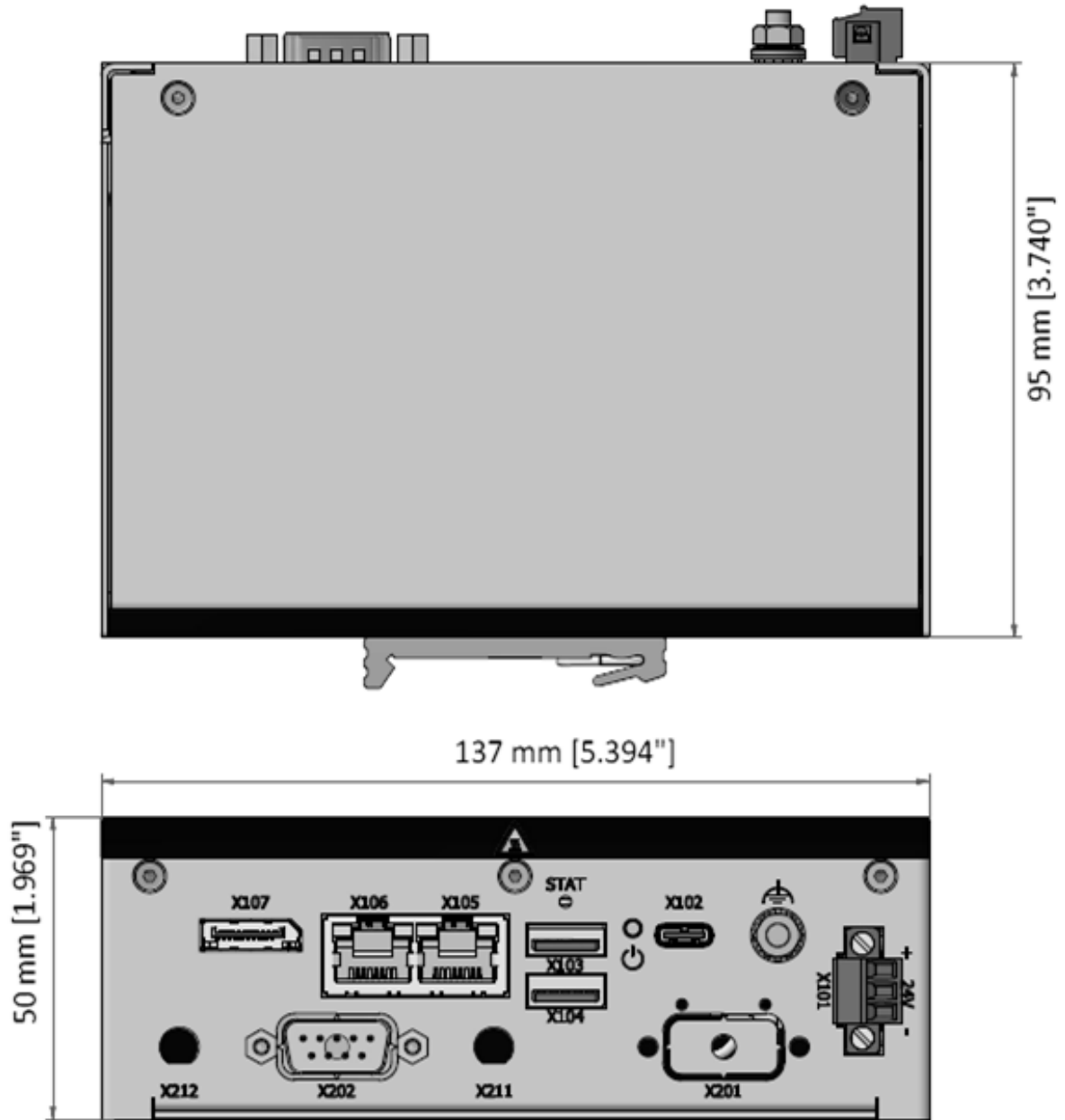
Figure 25: Mechanical Dimensions (mm)
