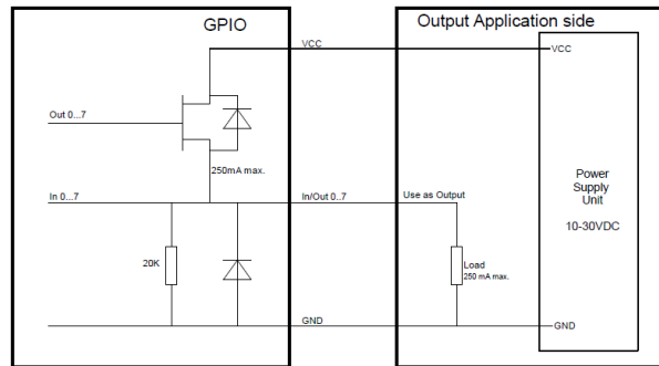
Figure 13: Output Application Connected to GPIO
