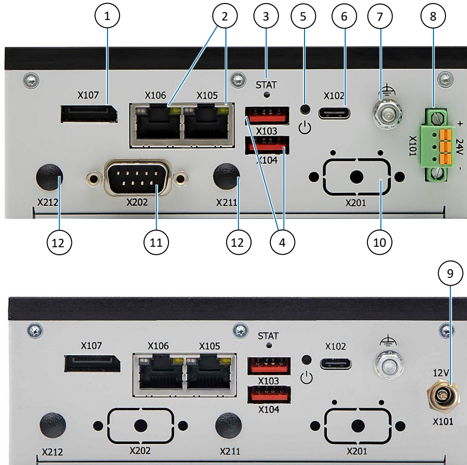
Figure 3: Front Panel
