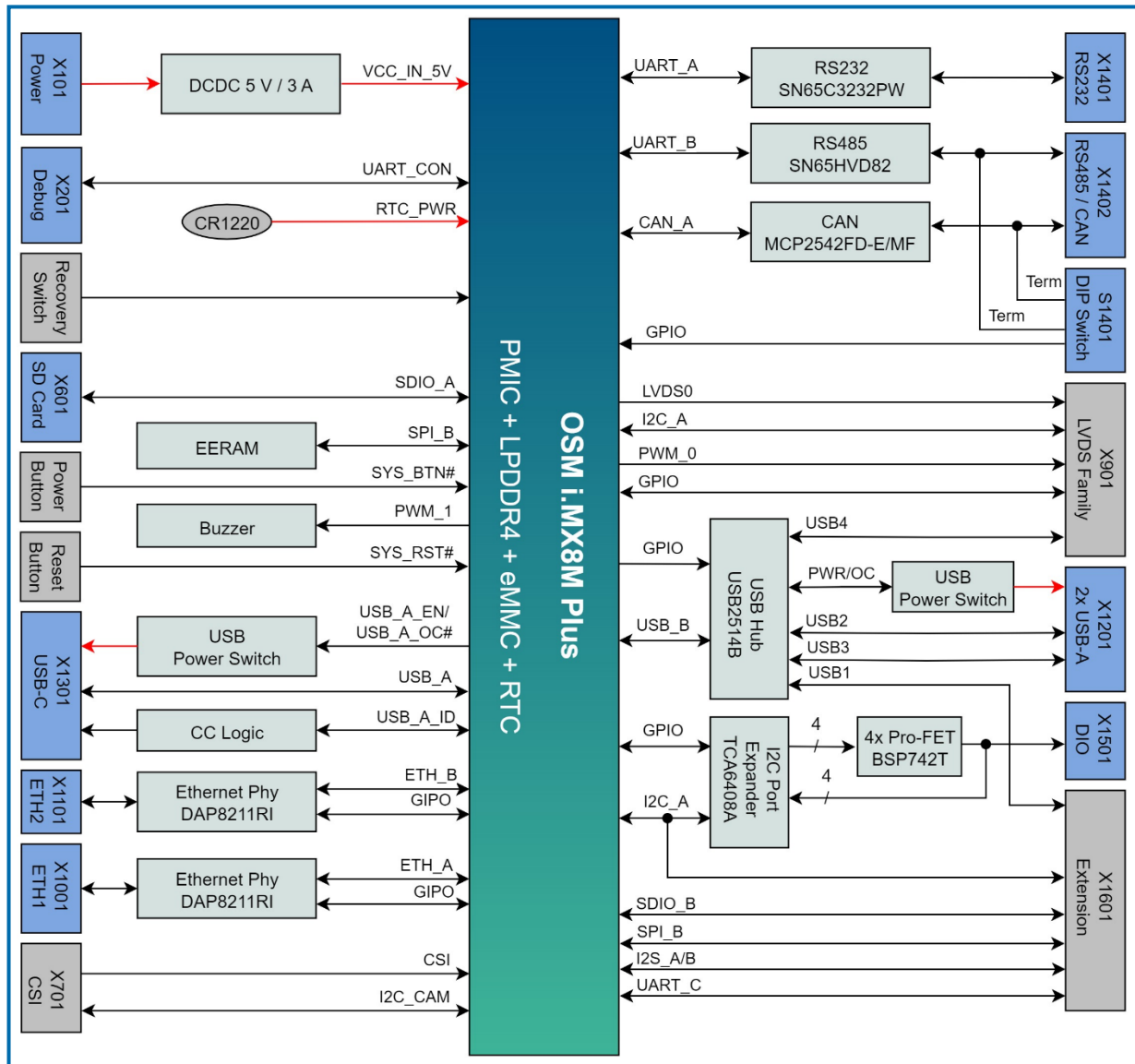
Figure 6: Block Diagram
