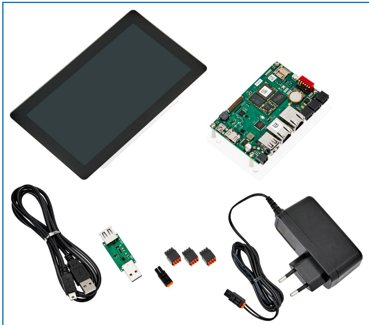
Figure 3: Development Kit DK i.MX8M Plus QC and DK 7" i.MX8M Plus QC
