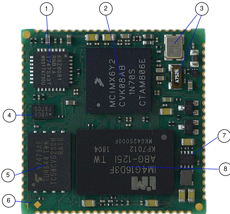
Figure 3: Top View
