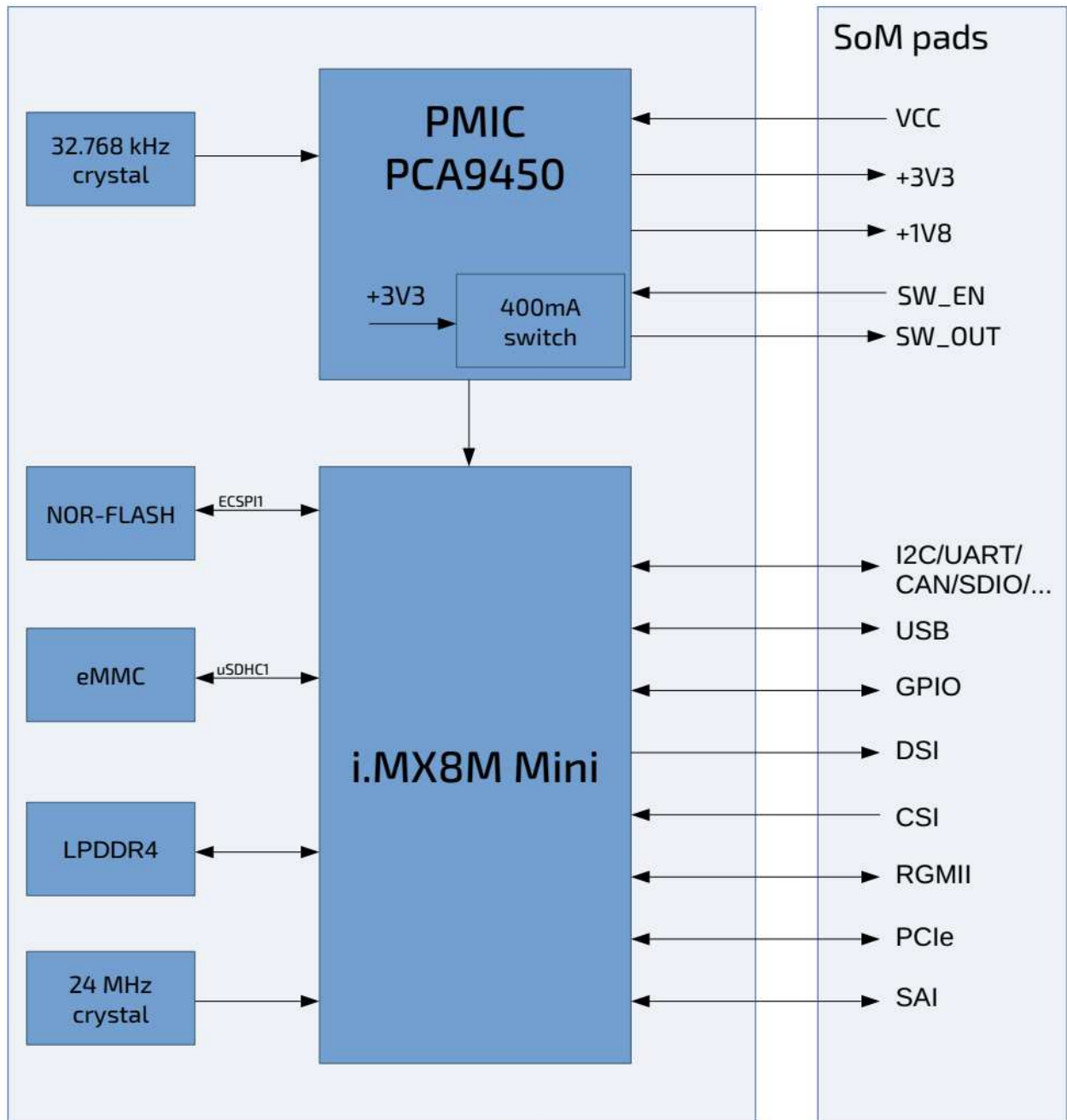
Figure 2: Block Diagram
