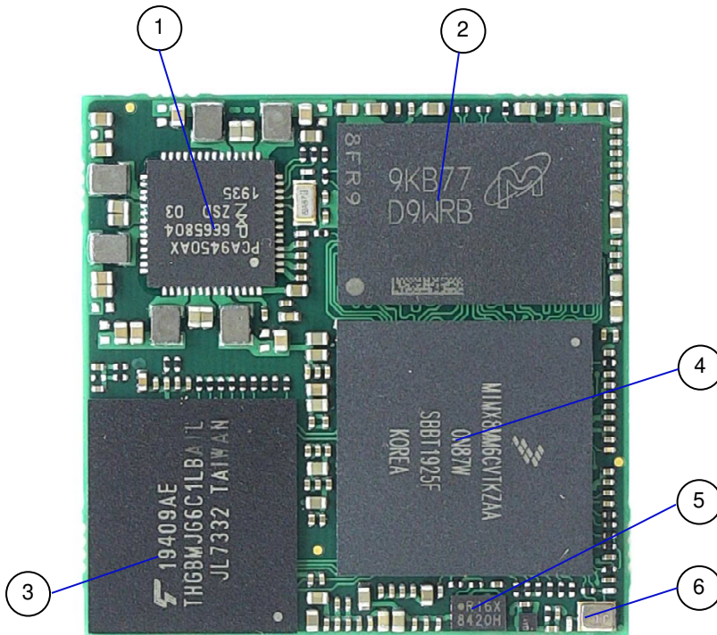
Figure 3: Top View
