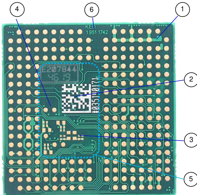
Figure 4: Bottom View
