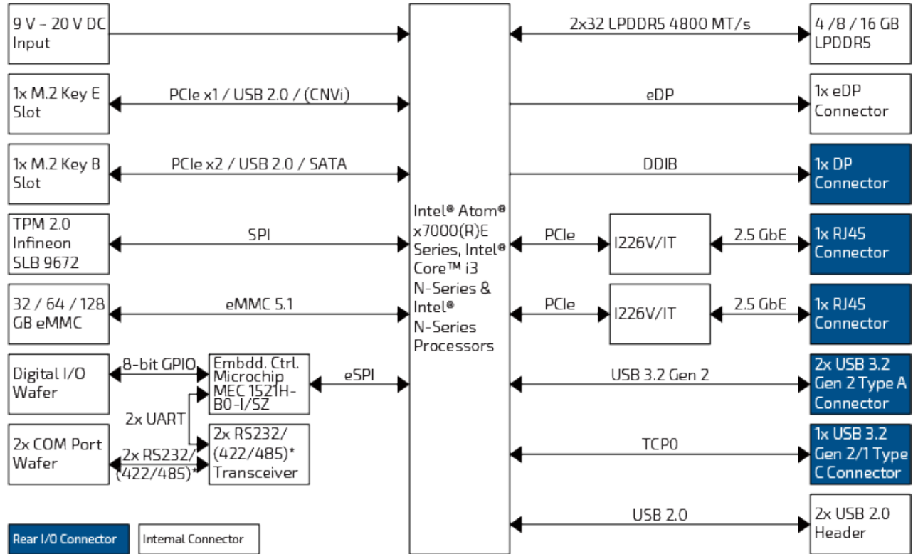
Figure 1: System Block Diagram 2.5"-SBC-AML/ADN
