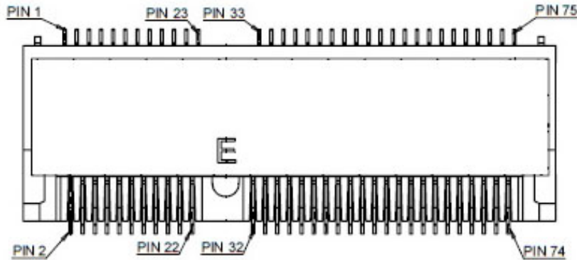
Figure 32: M.2 Key E 2230 Slot M2E1
