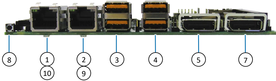
Figure 6: Connector Panel Side – 3.5"-SBC-RPH
