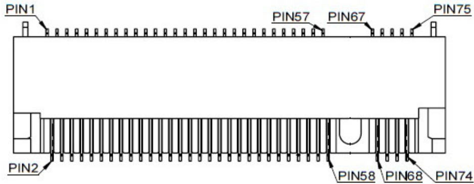
Figure 33: M.2 Key M 2280 Slot M2M1
