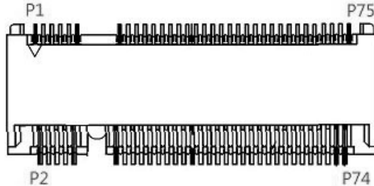
Figure 31: M.2 Key B 2242 / 3042 / 3052 / 2280 Slot M2B1
