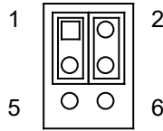
Figure 41: eDP / LVDS Backlight & Panel Power Selection JP4
