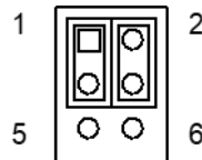
Figure 40: eDP / LVDS Backlight Enable Voltage Selection JP3
