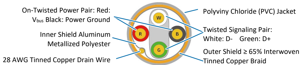
Figure 11: USB 2.0 High Speed Cable
