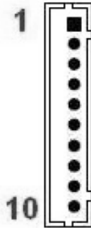
Figure 28: General Purpose Input / Output Header CN3
