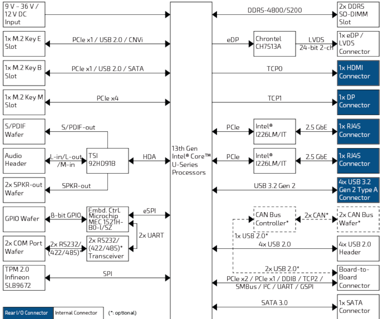
Figure 2: System Block Diagram 3.5"-SBC-RPH
