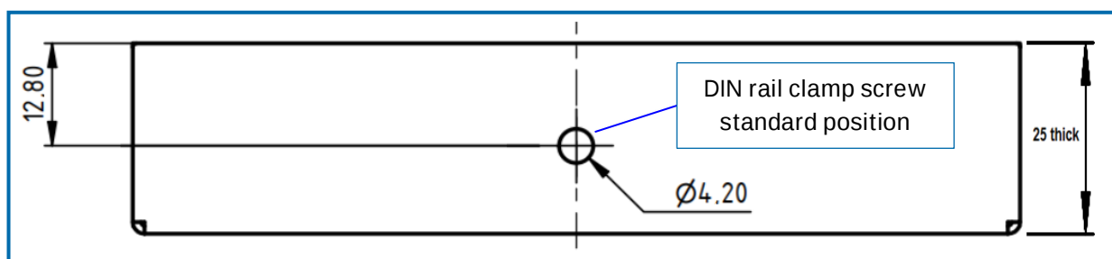
Figure 5: Rear View
