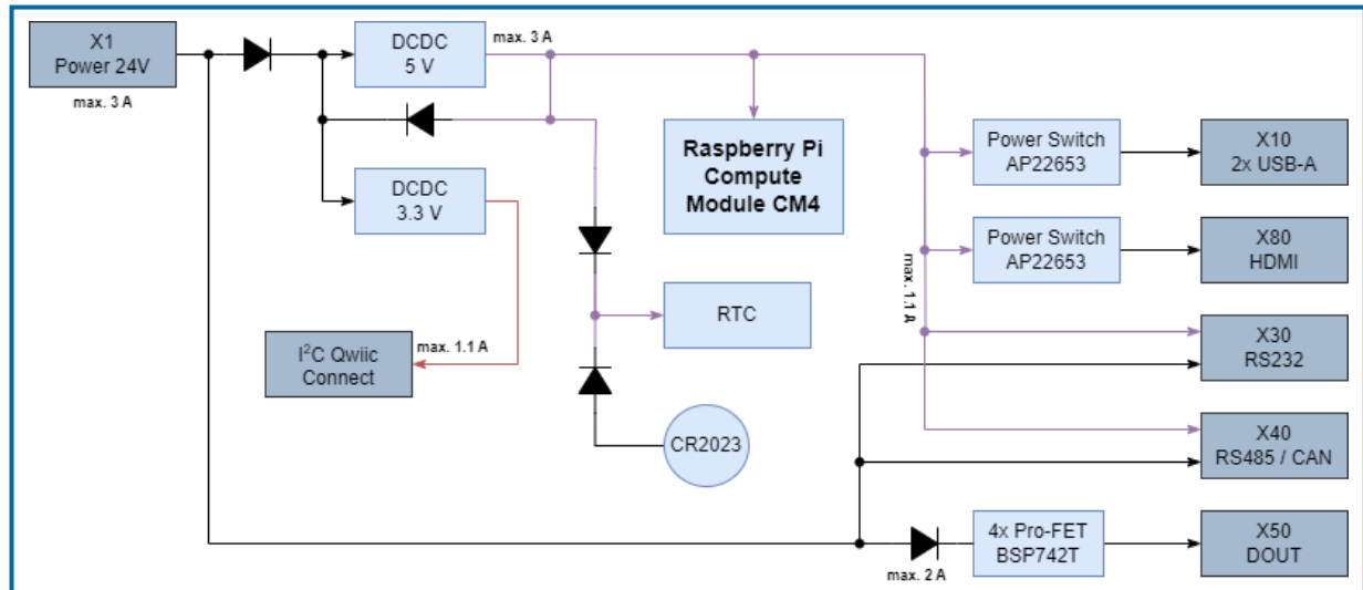
Figure 6: Power Tree
