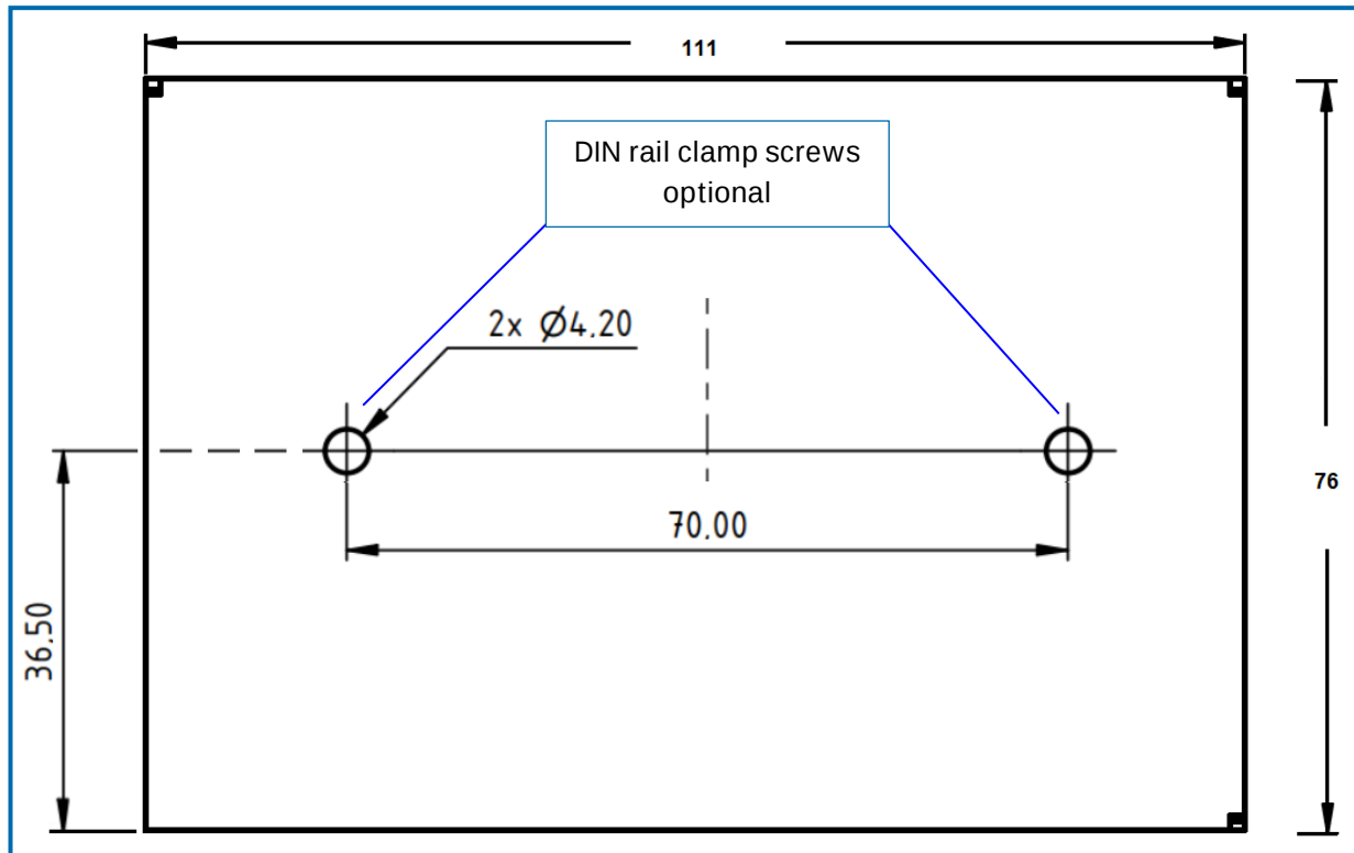
Figure 3: Bottom view
