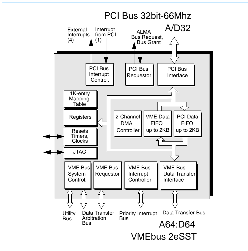
Figure 1 : ALMA2f block diagram
