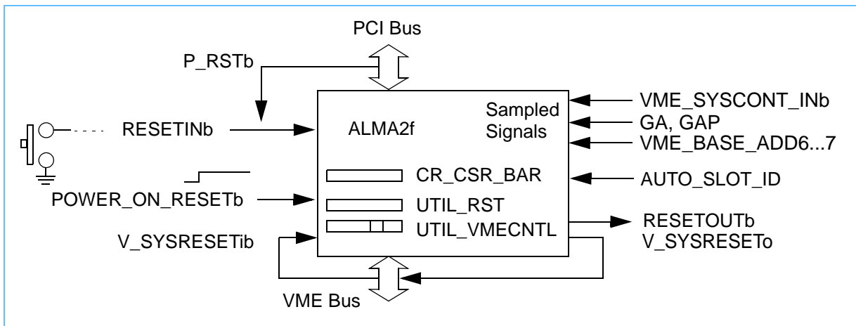
Schematic for Reset with ALMA2f
