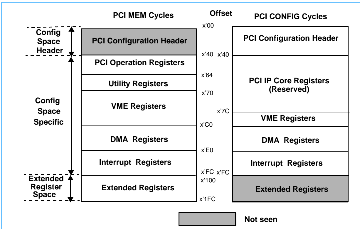
Figure 1-1. ALMA2f Configuration Space and Extended Space Register
