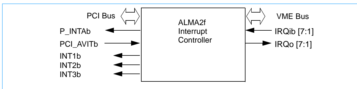
Figure 6-1. Interrupt Signals controlled by ALMA2f
