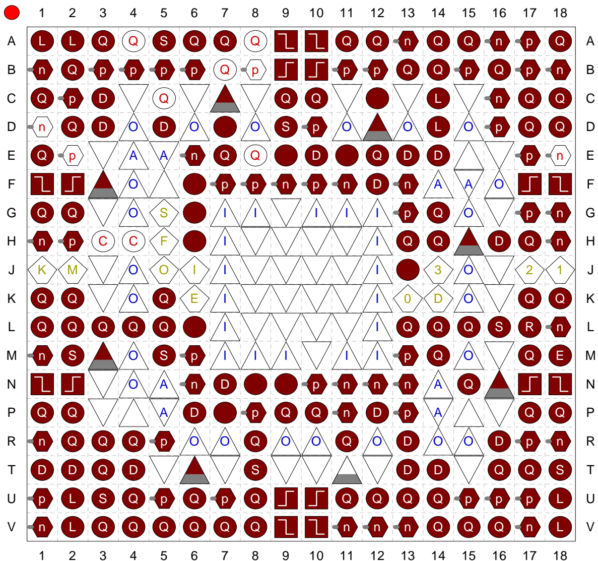
Figure 6 : Top view EPC325F324I7
