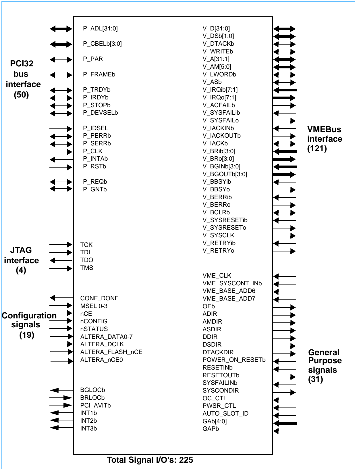
Figure 5 : ALMA2f Signal Pins block diagram
