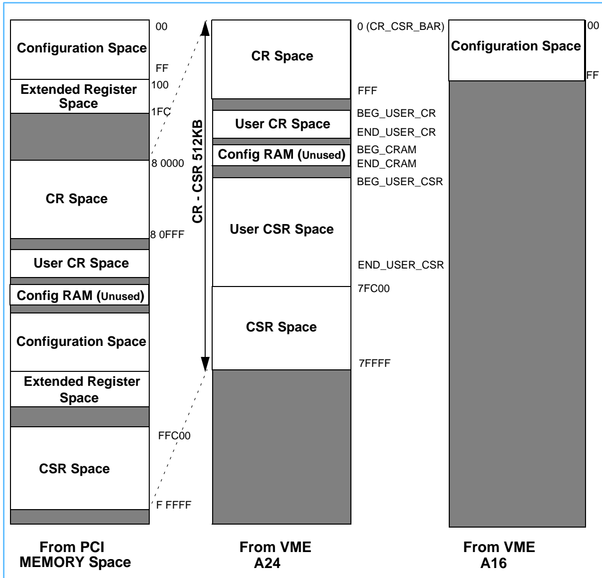
Figure 4 : ALMA2f Addressing Model.
