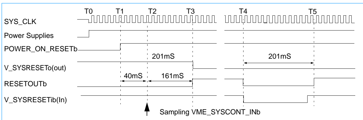
Figure 5-1. PowerOn Reset with ALMA2f
