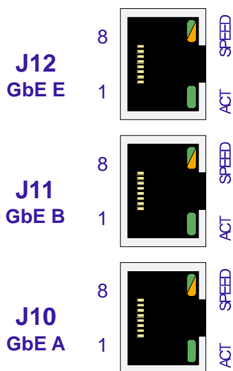
Figure 2-4: GbE Con. J10, J11 and J12
