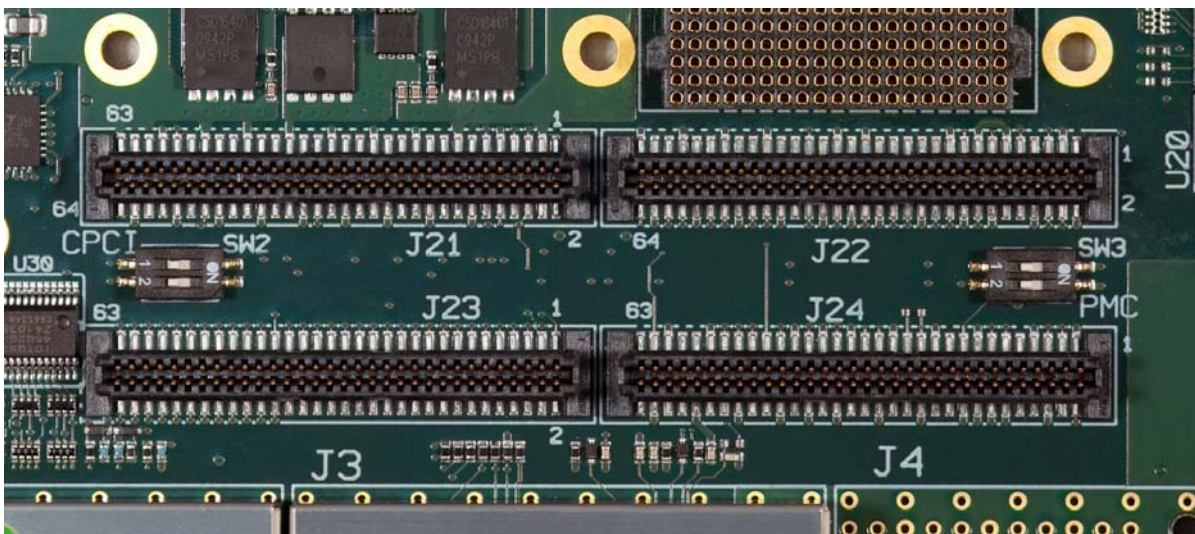
Figure 4-2: DIP Switches SW2 and SW3
