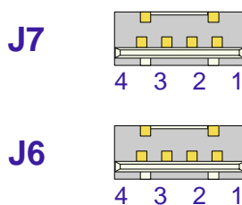
Figure 2-1: USB Con. J6 and J7
