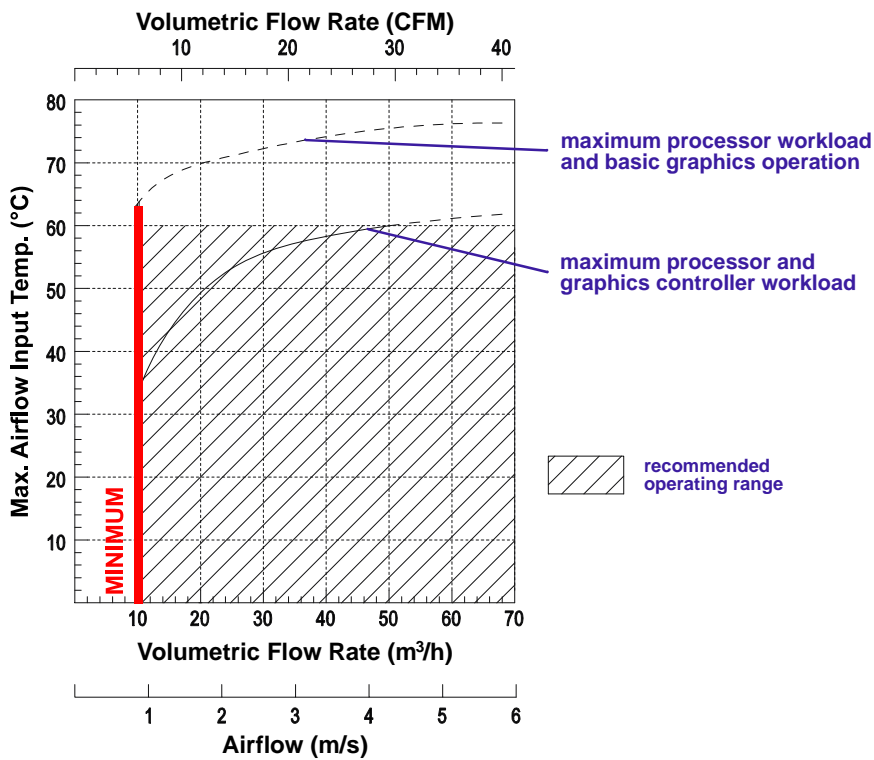
Figure 6-4: CP6004-SA with Core™ i5-3610ME (SV) 2.7 GHz
