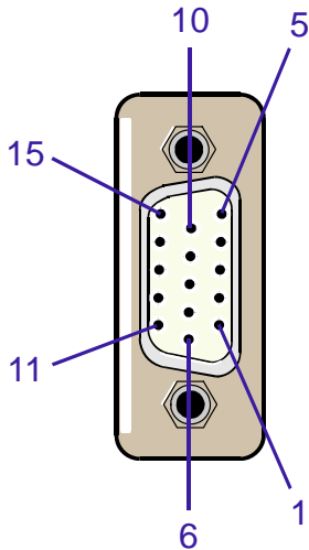
Figure 2-2: D-Sub VGA Con. J9 Table 2-11: D-Sub VGA Connector J9 Pinout
