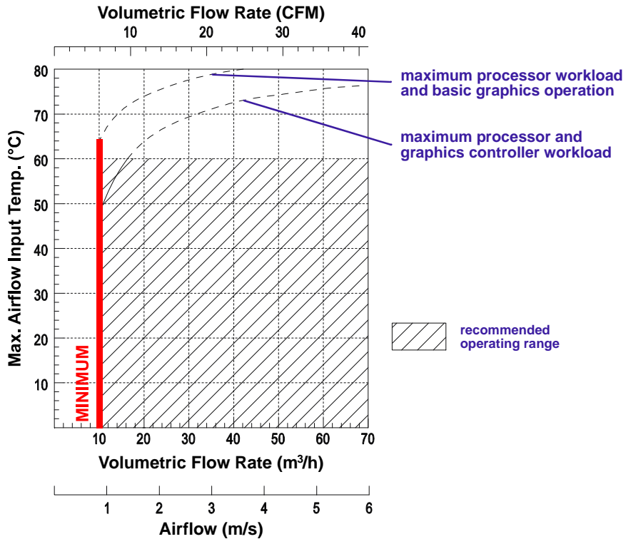
Figure 6-2: CP6004-SA with Core™ i7-3612QE (SV) 2.1 GHz
