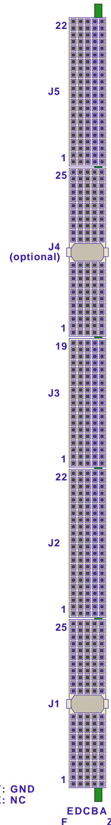
Figure 2-8: CompactPCI Con. J1-J5
