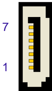
Figure 2-5: SATA Con. J14
