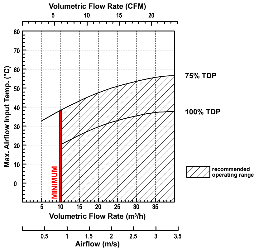
Figure 6-4: Operating Limits: Core™ 2 Duo 2.16 GHz, Wide Heat Sink
