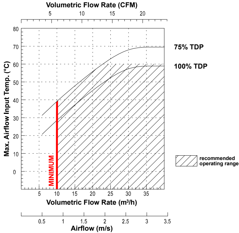
Figure 6-6: Operating Limits: Core™ Duo 2.0 GHz, Narrow Heat Sink
