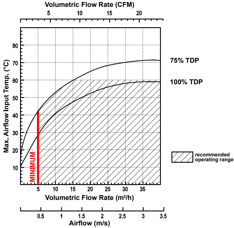
Figure 6-2: Operating Limits: Core™ Duo 2.0 GHz, Wide Heat Sink
