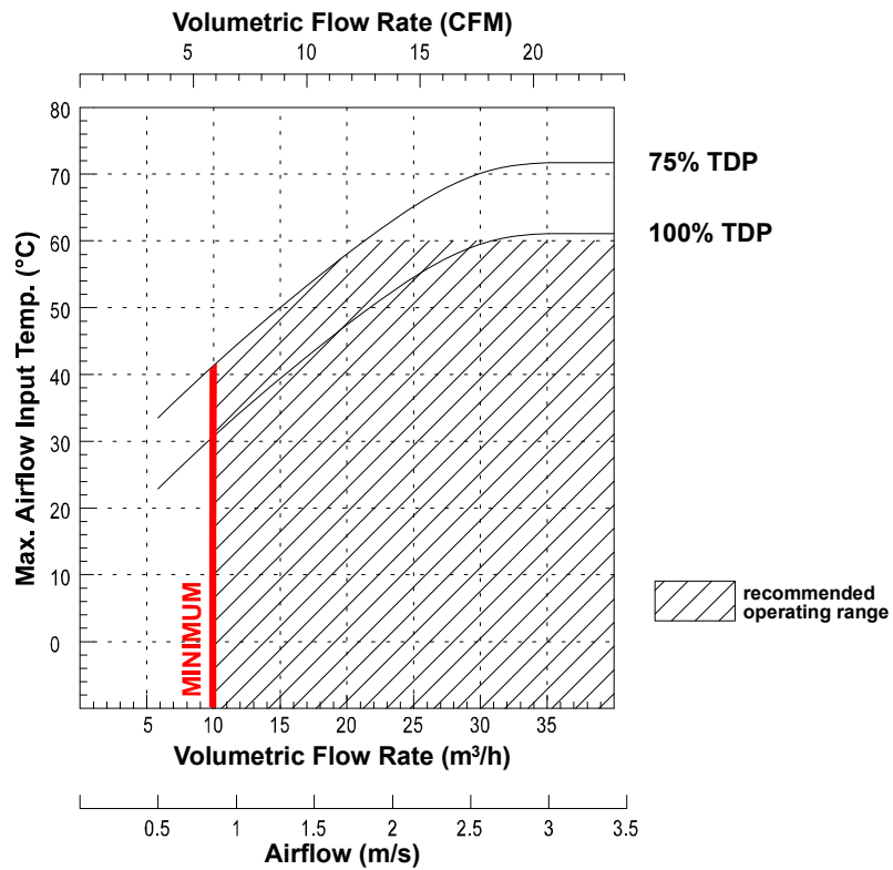
Figure 6-6: Operating Limits: Core™ Duo 2.0 GHz, Narrow Heat Sink
