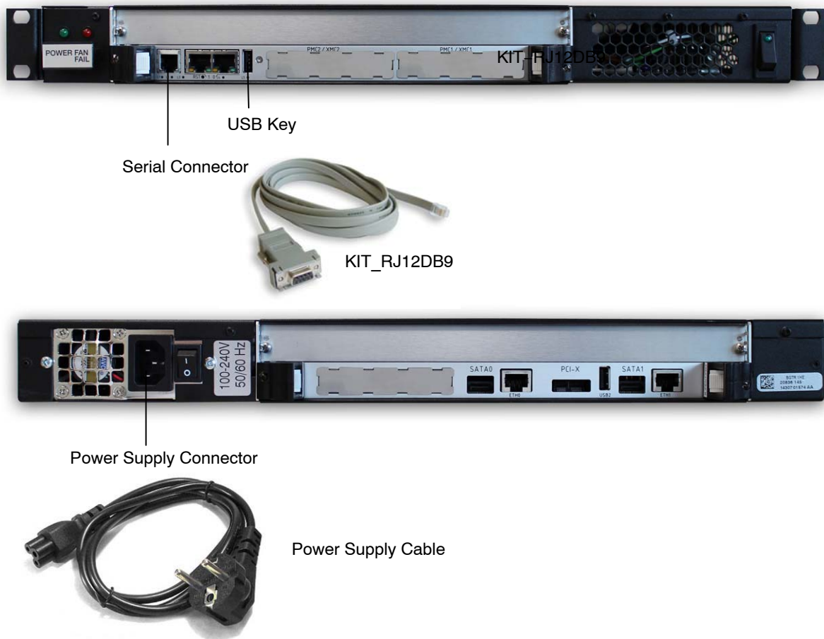
Figure 6: Connecting Easy VM6050
