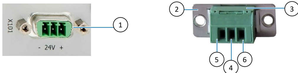
Figure 19: Power IN Connector and Mating Power IN Connector
