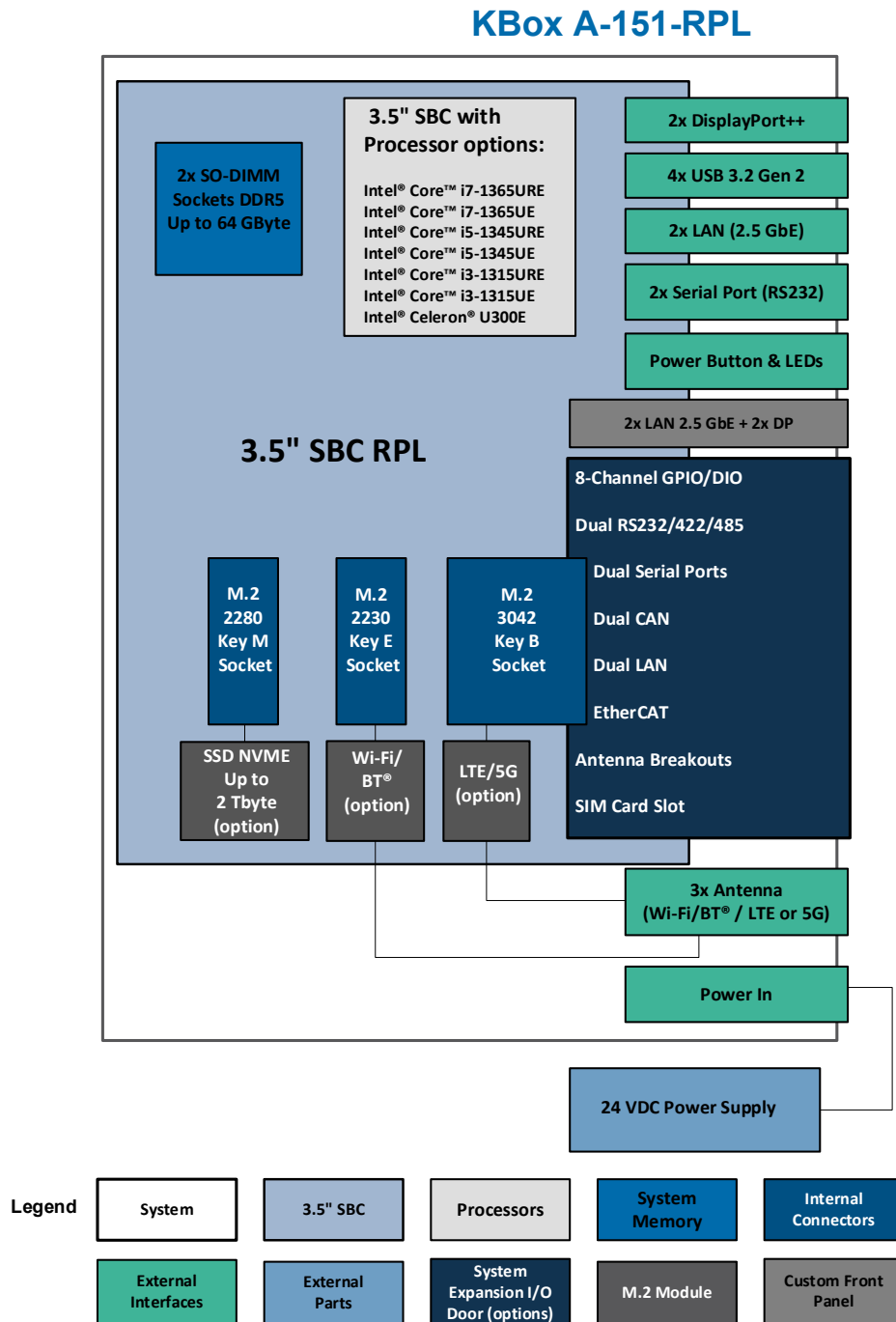
Figure 20: Block Diagram KBox A-151-RPL
