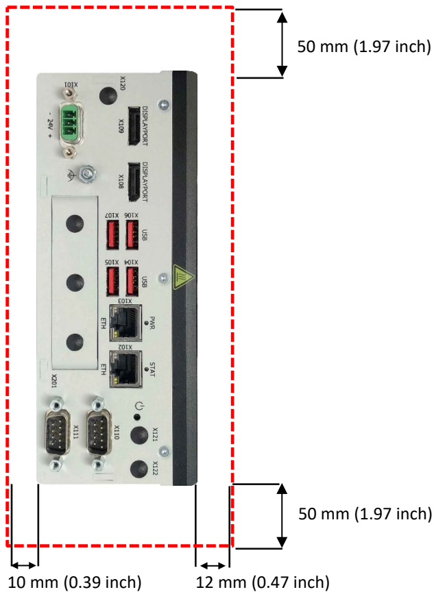
Figure 18: Keep Out Areas- Vertical
