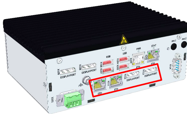
Figure 13: Custom Front Panel with Dual Ethernet and Dual DP Ports
