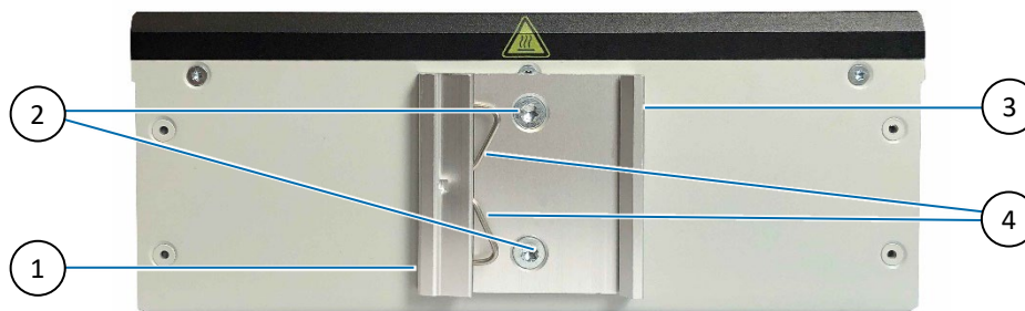
Figure 14: DIN Rail Clamp (50 mm x 50 mm)
