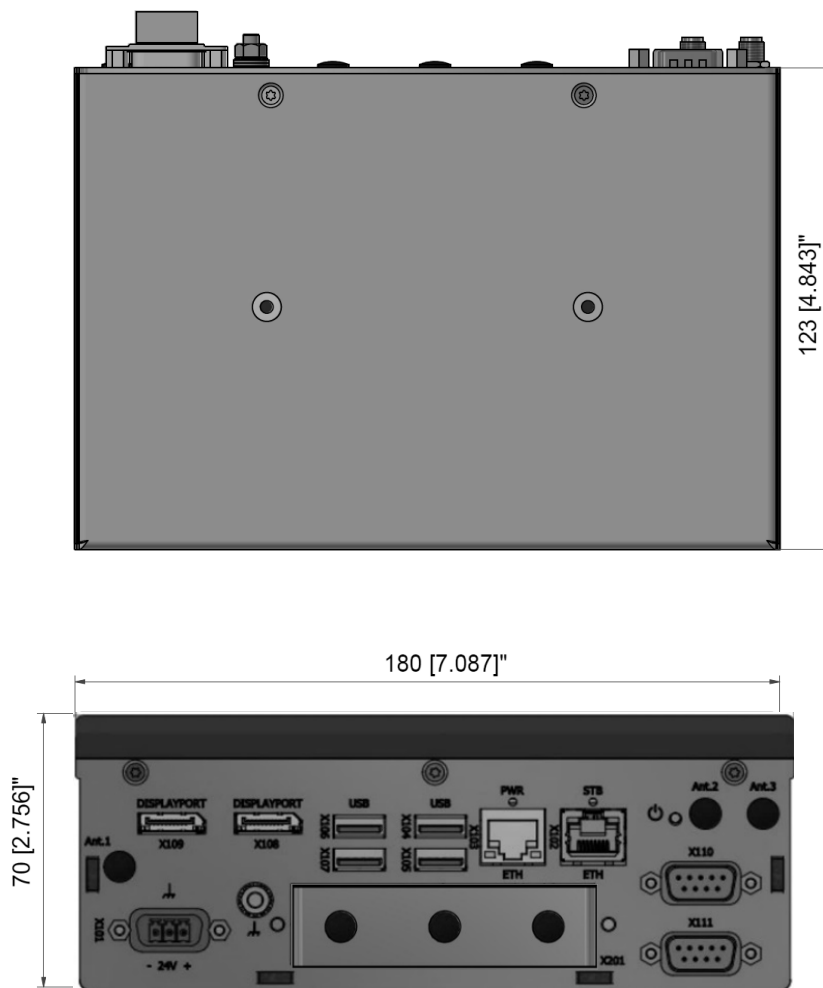
Figure 21: Mechanical Dimensions (mm)
