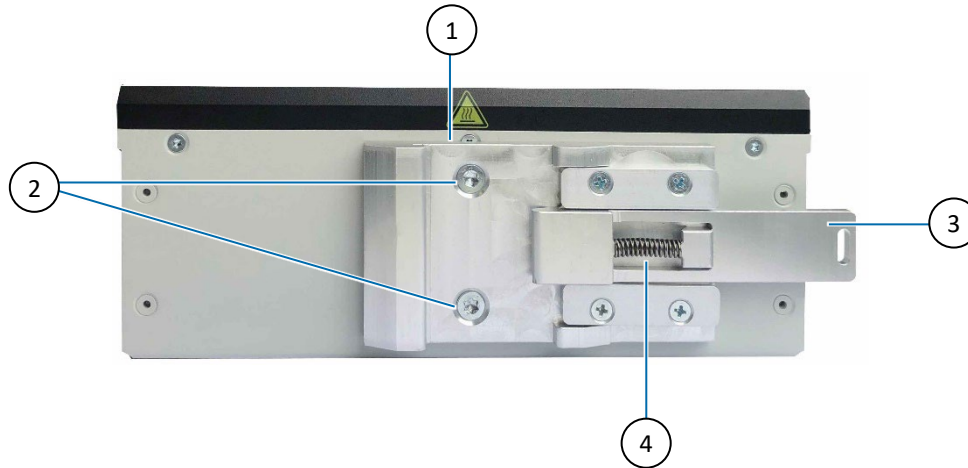
Figure 16: Rugged DIN Rail Clamp
