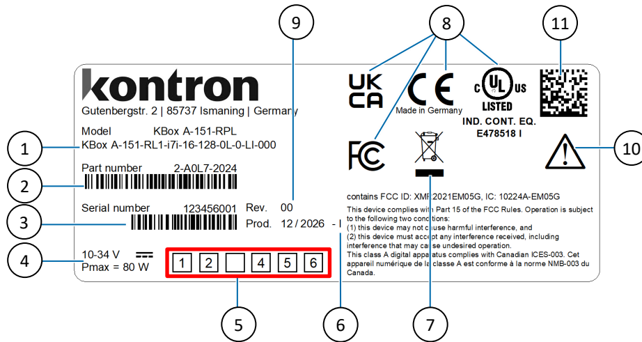
Figure 2: Type Label Example
