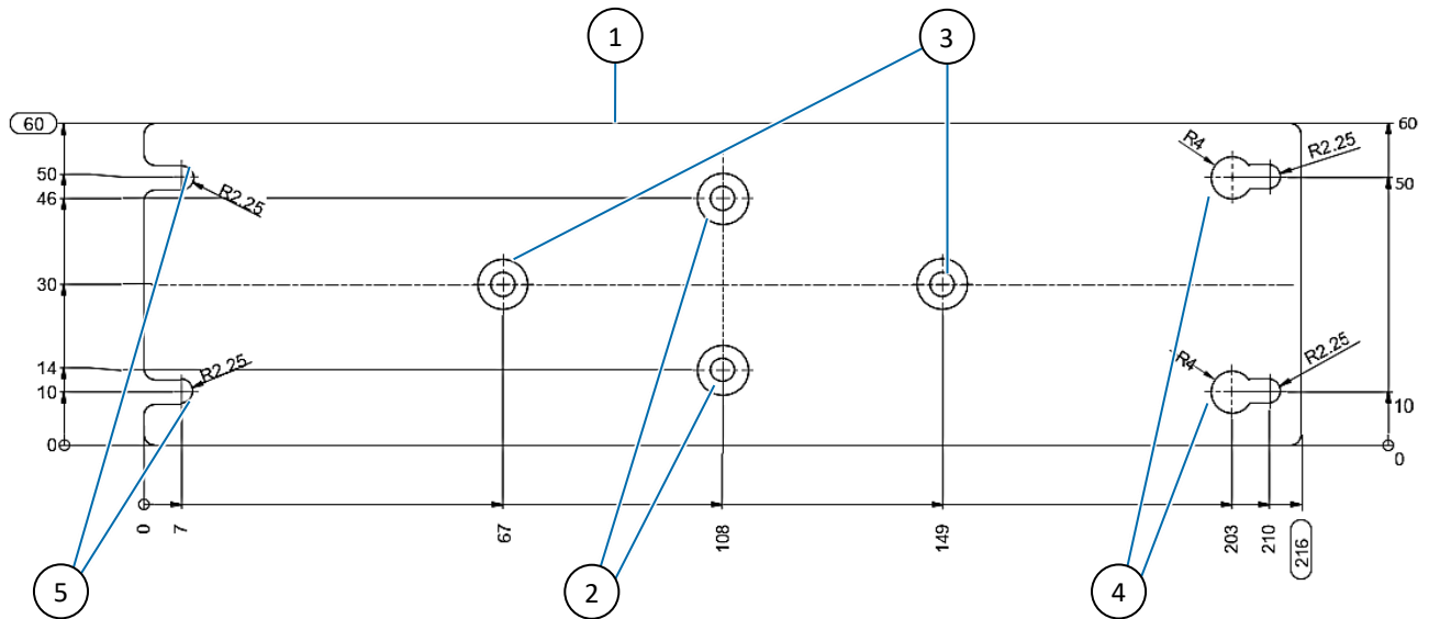
Figure 17: Book Mount Bracket
