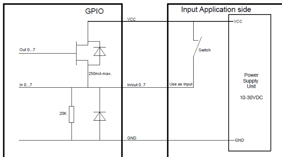
Figure 13: Input Application Connected to GPIO
