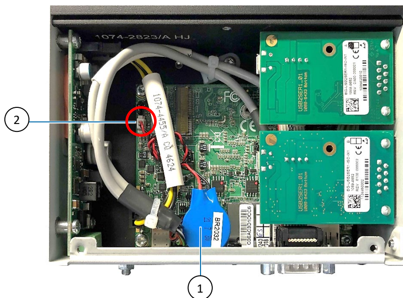
Figure 33: RTC Lithium Battery and Battery Header
