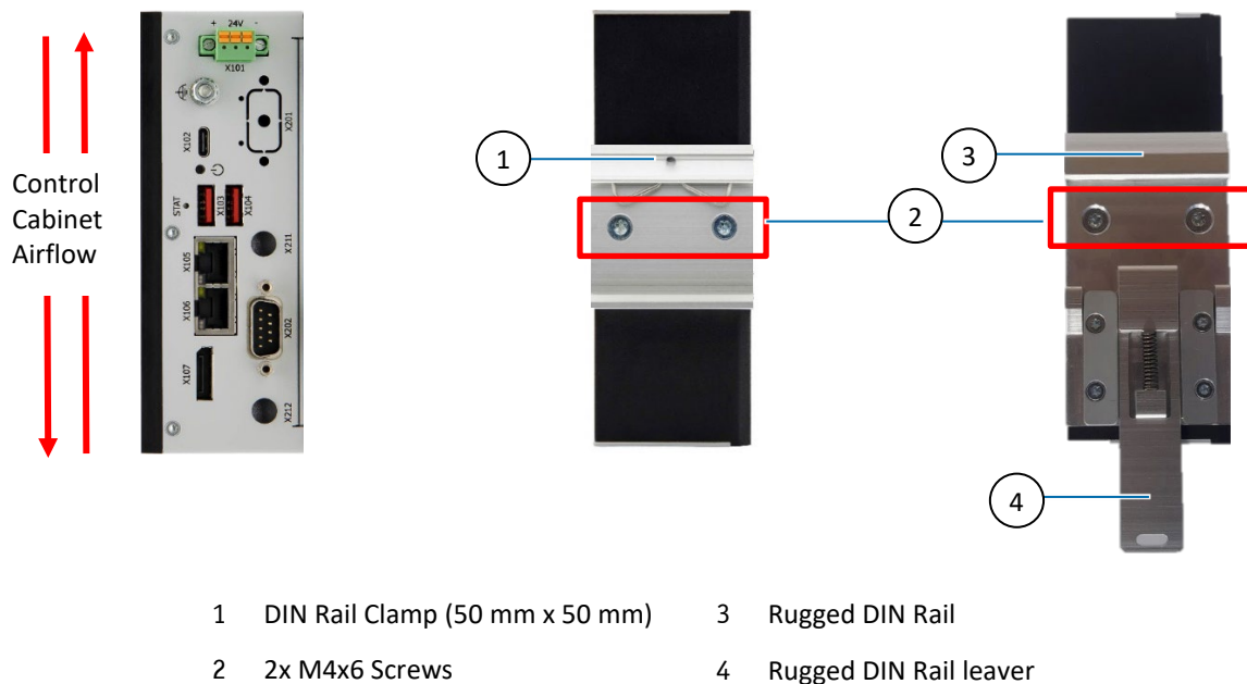
Figure 19: DIN Rail Clamp and Rugged DIN Rail Clamp (default position)
