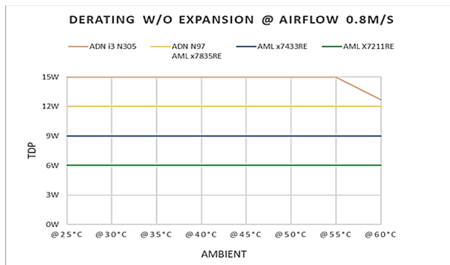
Figure 15: Derating TDP versus Temperature Curves (without expansion & airflow 0.8 m/s)
