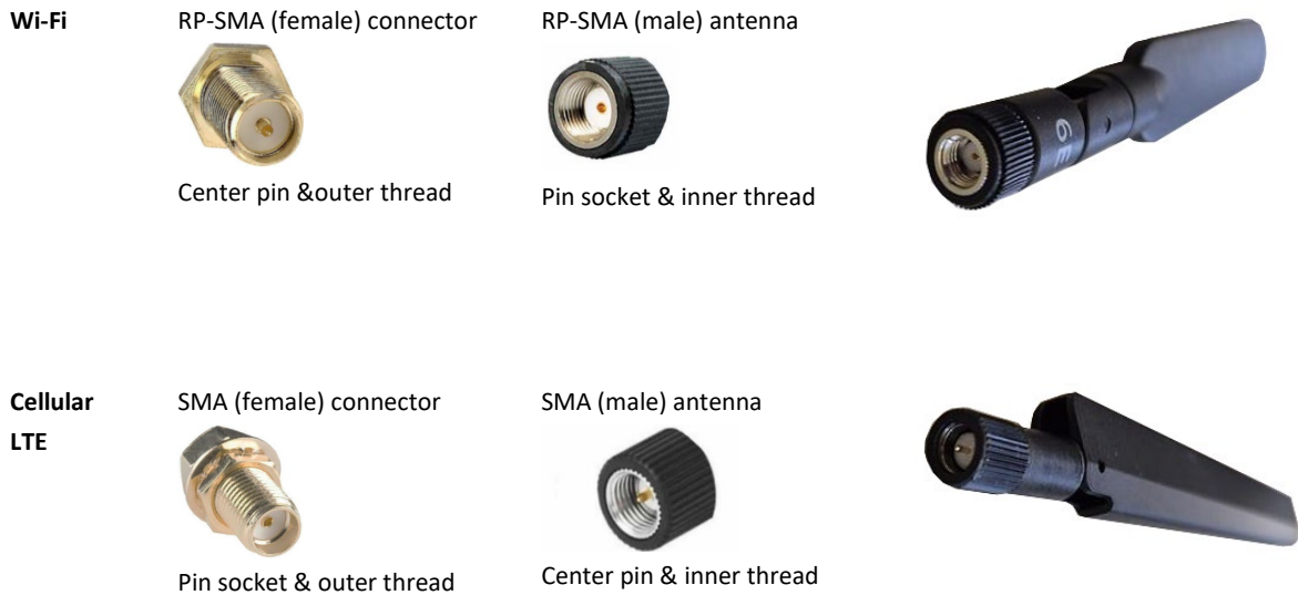
Figure 4: Wi-Fi and Cellular LTE Connectors and Antenna Type
