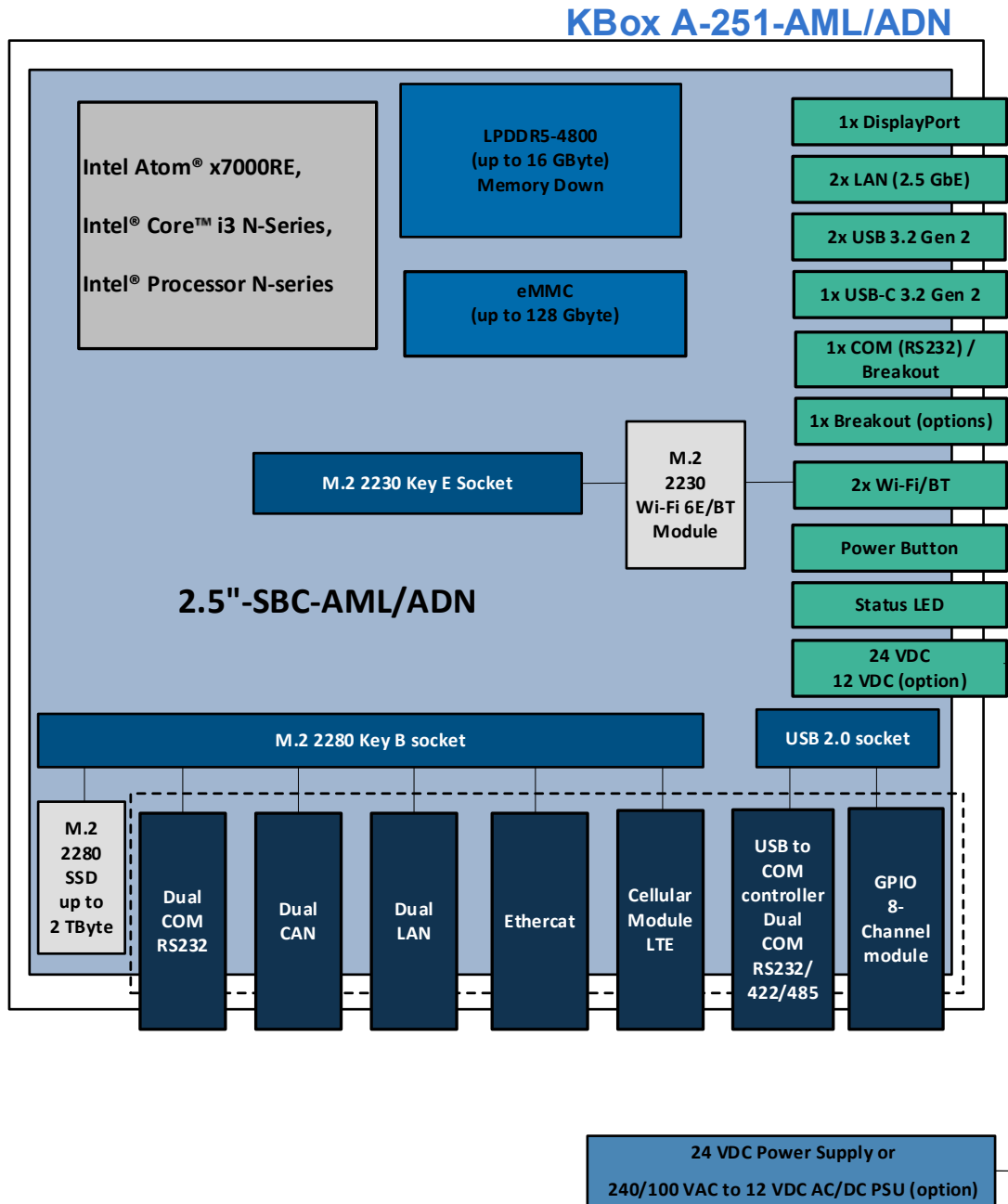
Figure 24: Block Diagram - KBox A-251-AML/ADN
