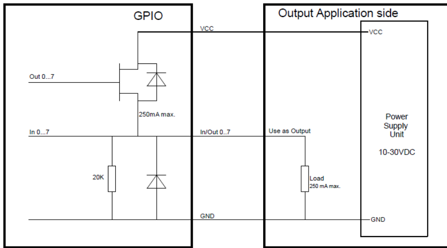
Figure 14: Output Application Connected to GPIO
