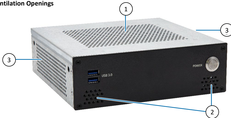
Figure 10: Ventilation Openings
