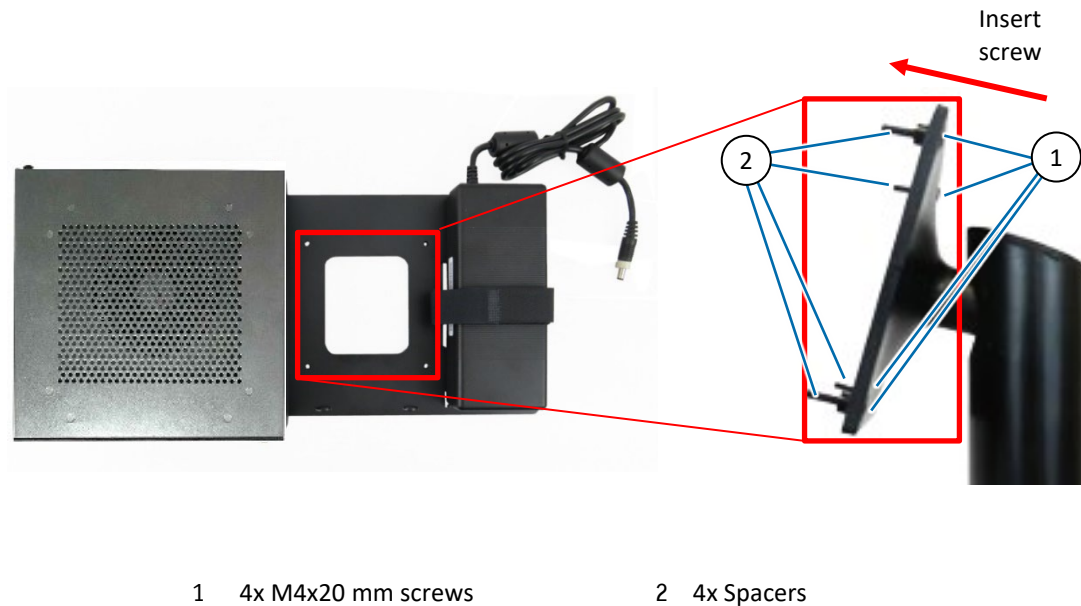
Figure 18: Mounting with a VESA Stand on the Monitor
