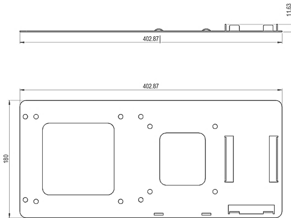
Figure 25: VESA 100 Mount Dimensions (mm)
