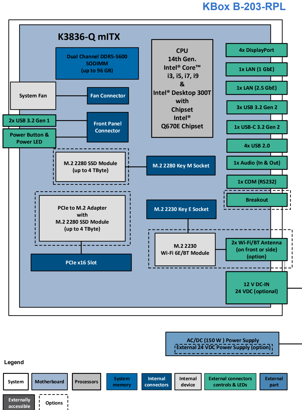
Figure 22: Block Diagram KBox B-203-RPL
