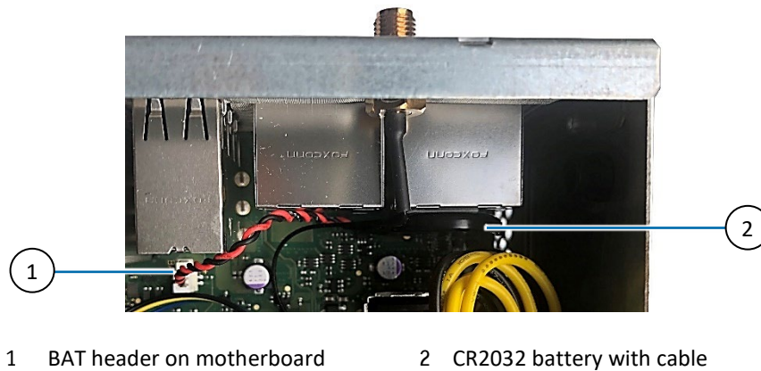
Figure 28: CR2032 Lithium Battery and BAT header
