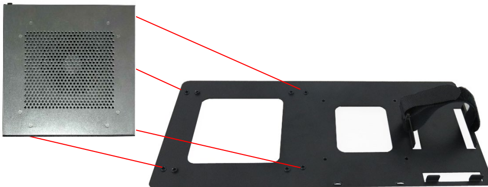
Figure 14: KBox B-203-RPL Mounting Position
