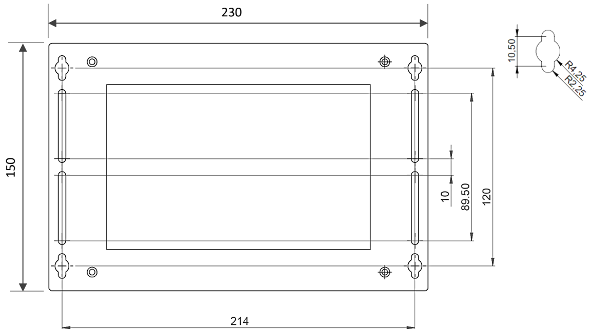
Figure 24: Wall Mount Dimensions (mm)
