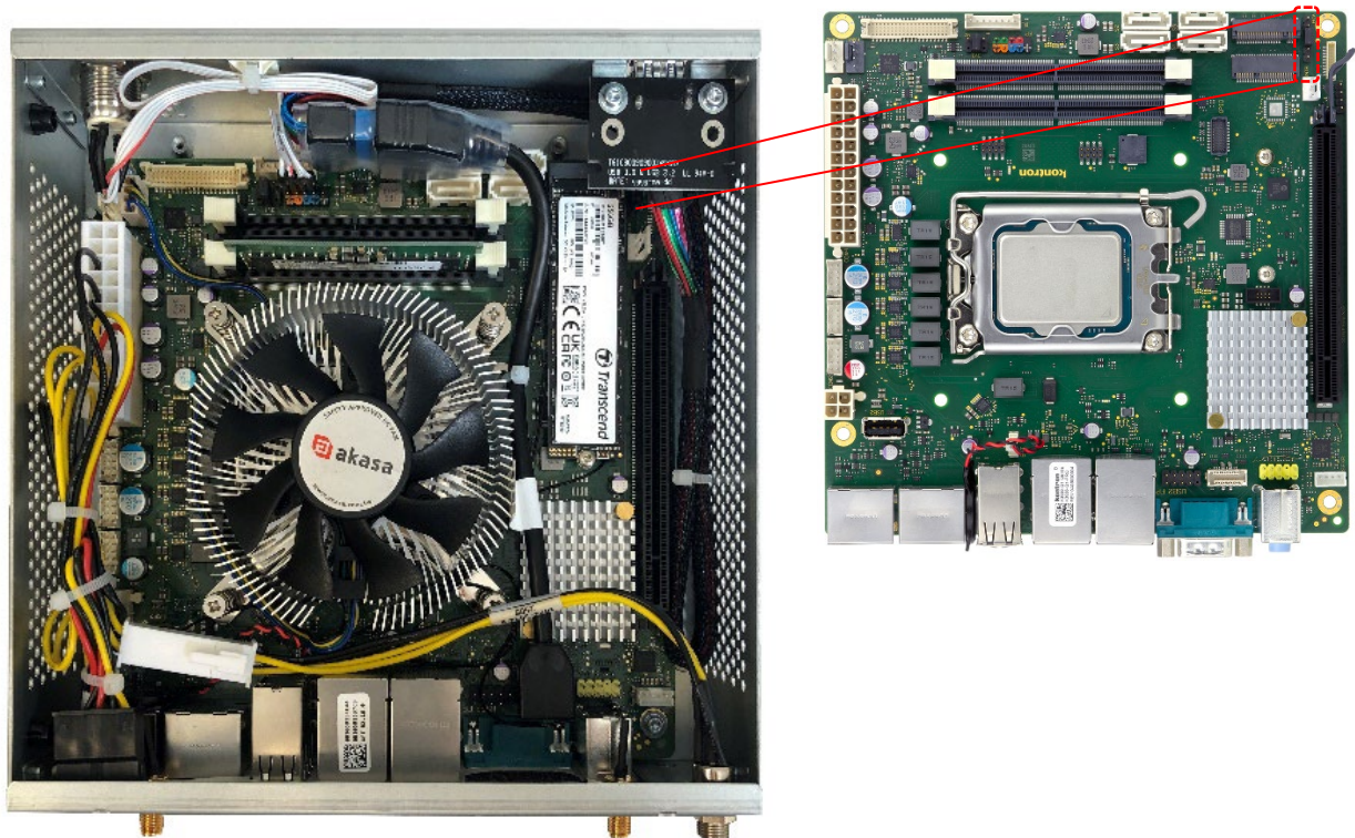
Figure 27: Configuration Jumper Header
