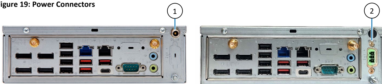
Figure 19: Power Connectors
