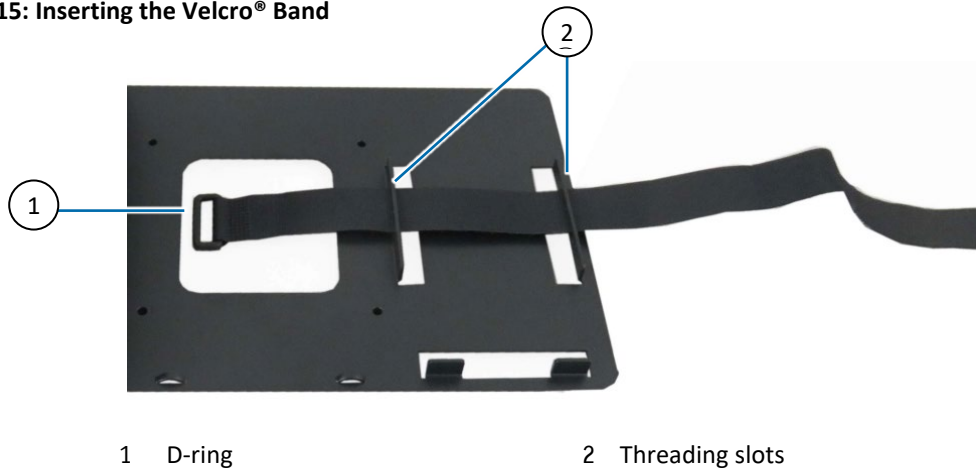
Figure 15: Inserting the Velcro® Band
