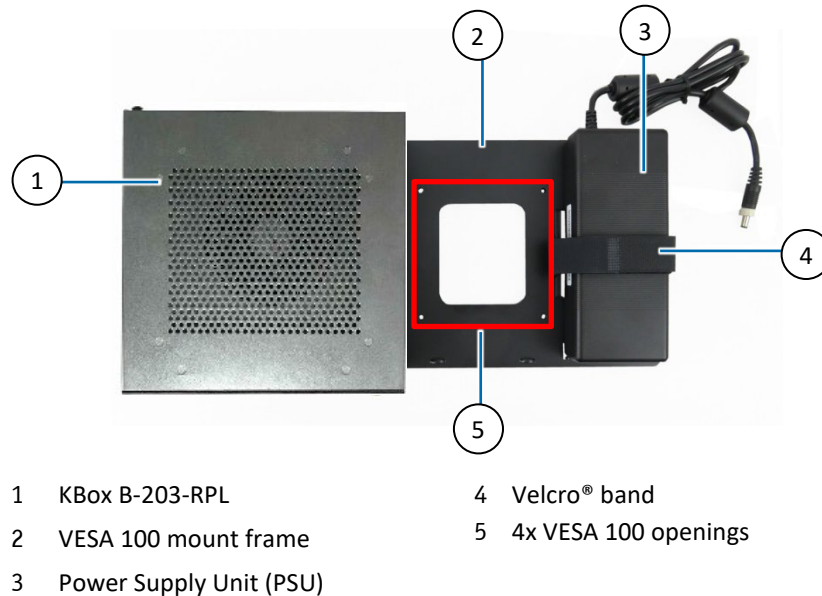
Figure 13: VESA 100 Mount Assembly
