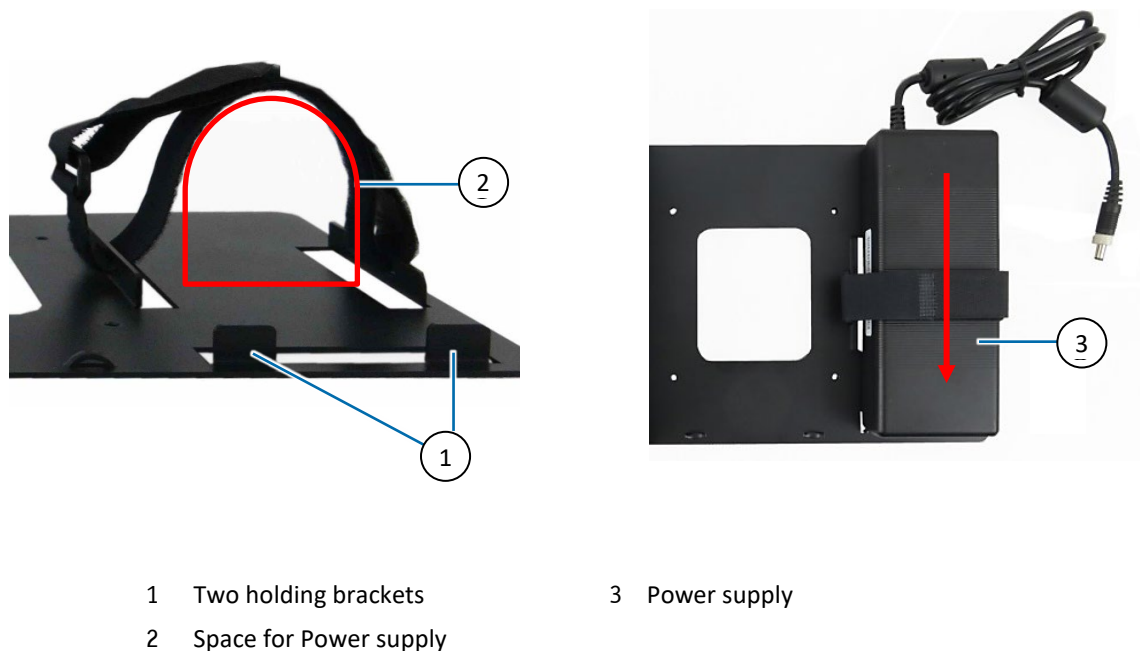
Figure 16: Positioning the Power Supply
