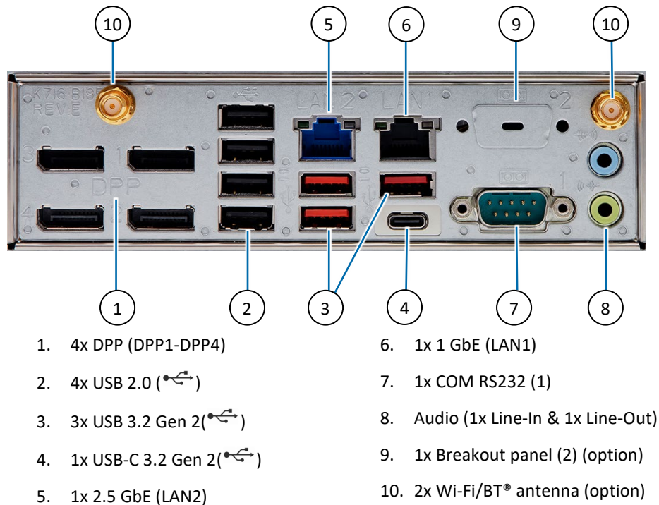
Figure 5: Interface Panel
