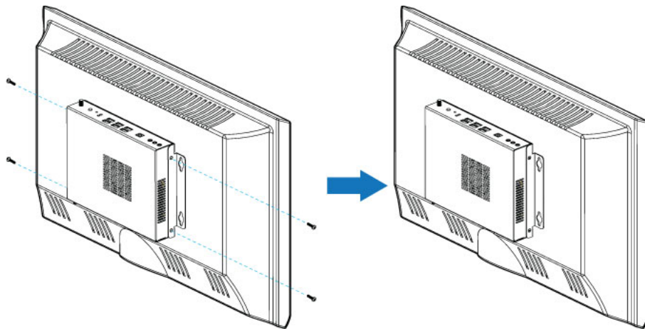
Figure 18: Securing the KBox F-210 Series and the mounting bracket together
