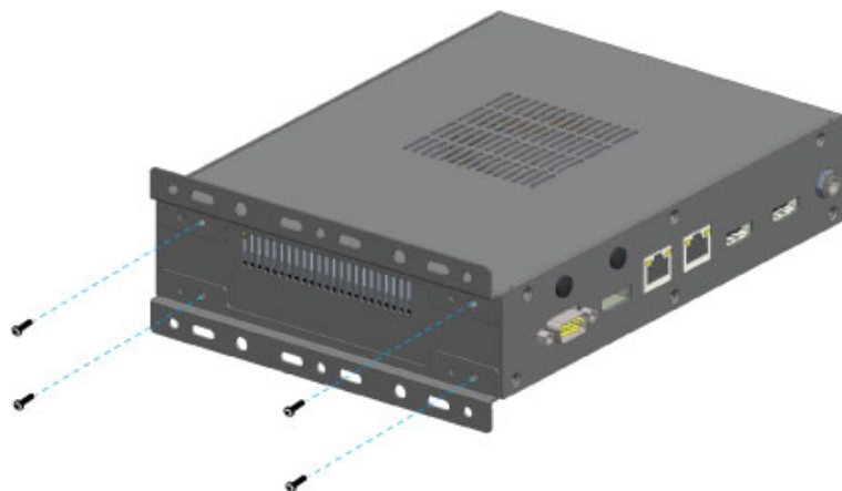
Figure 20: Securing the stand bracket pair to the KBox F-210 Series
