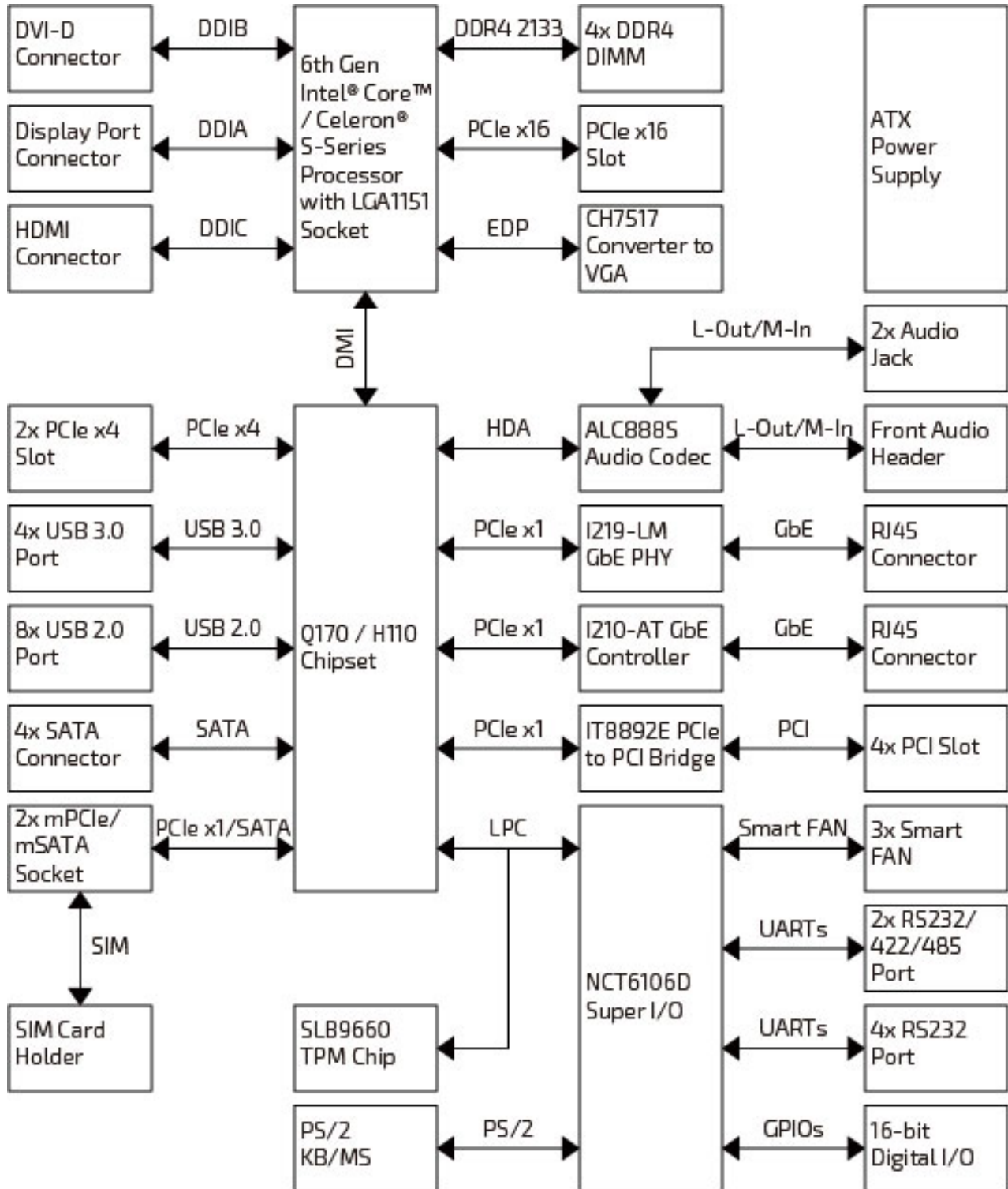
Figure 1: System Block Diagram ATX-SKL-S
