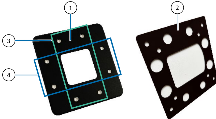
Figure 15: Portrait Adapter and Gasket
