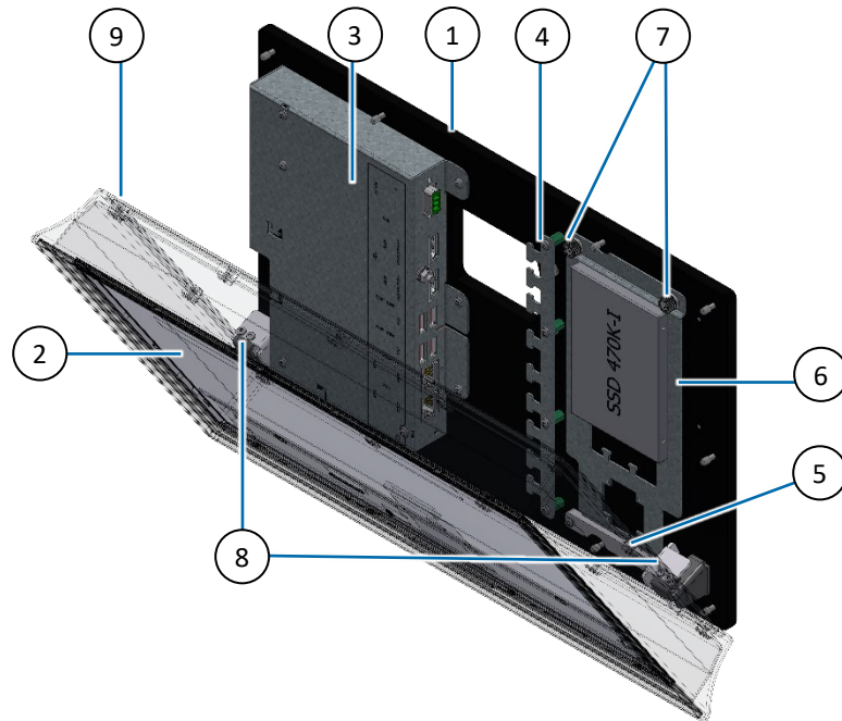
Figure 18: Opening and Closing the KPanel S-RPL
