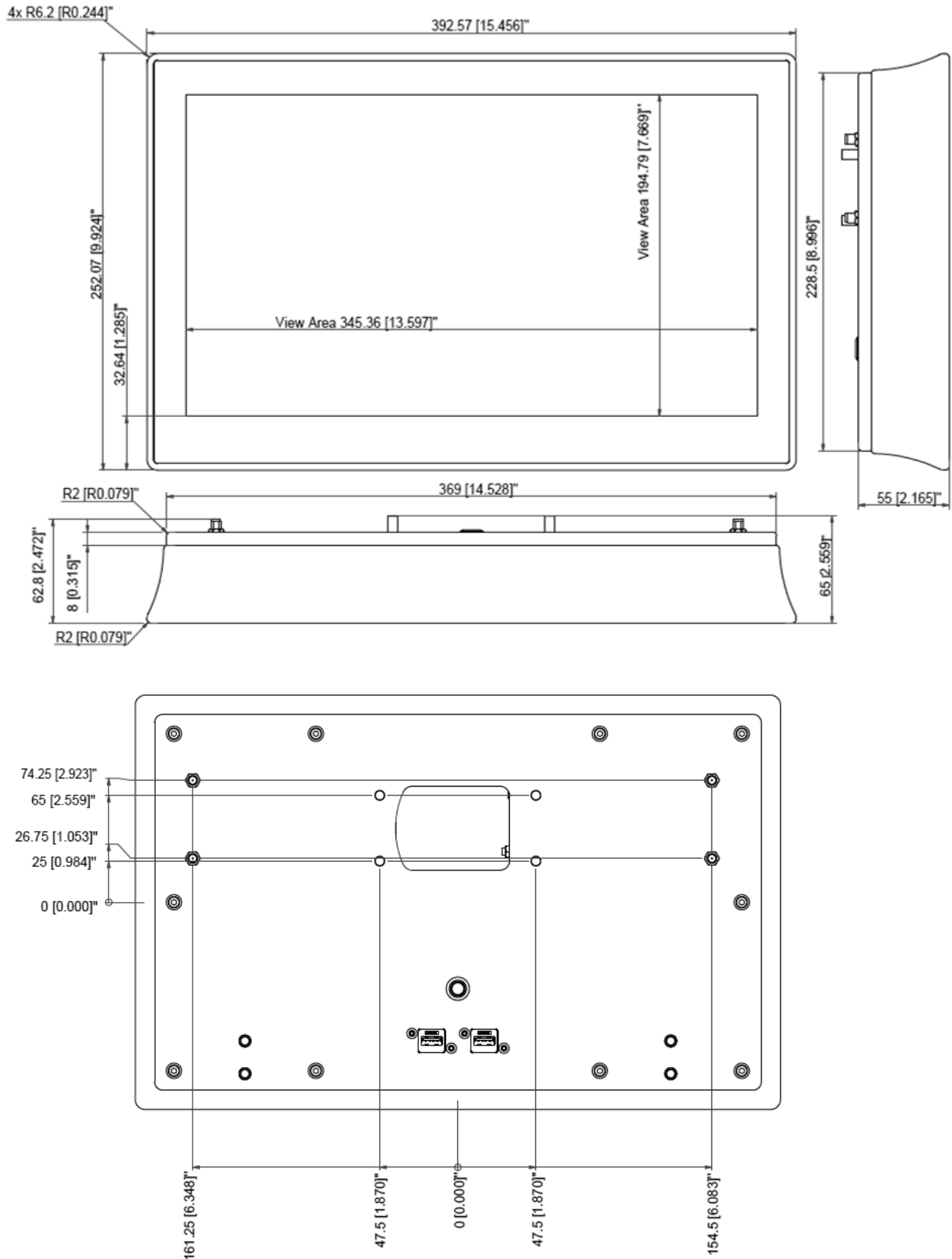
Figure 12: 15.6" Dimension Diagram (mm/inch)
