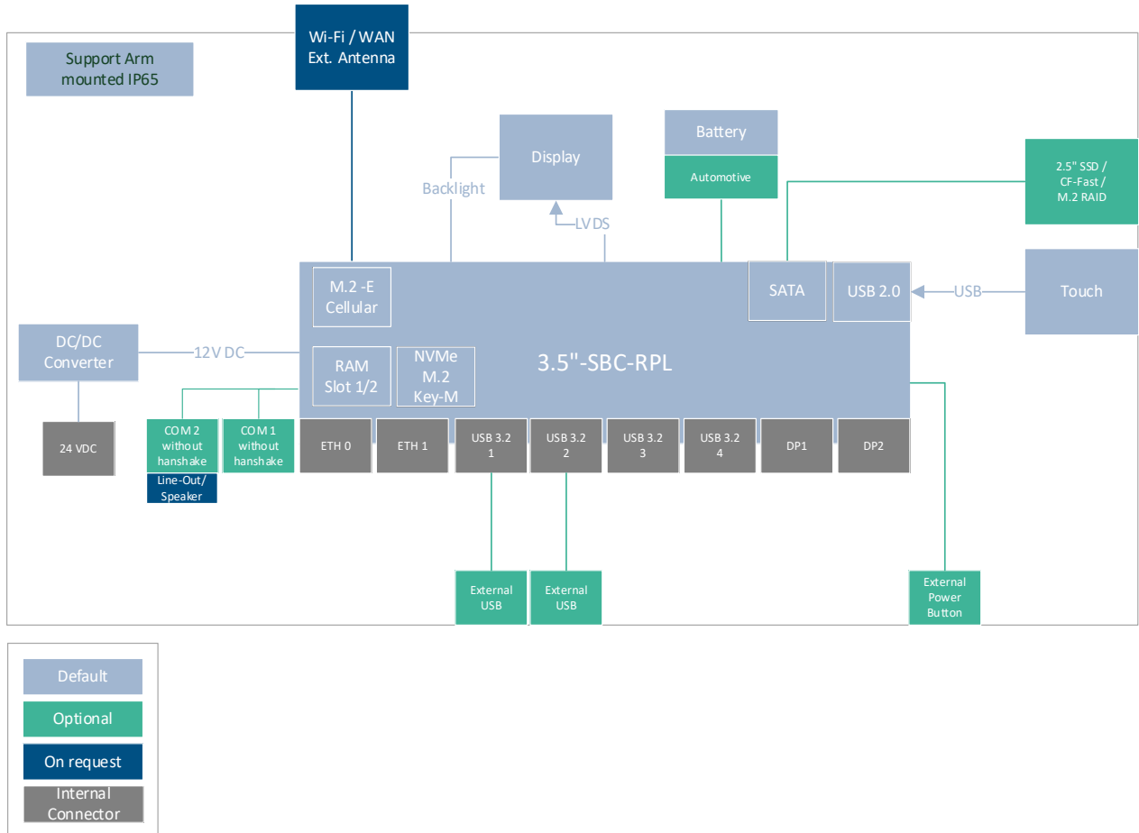
Figure 9: Block Diagram KPanel S-RPL
