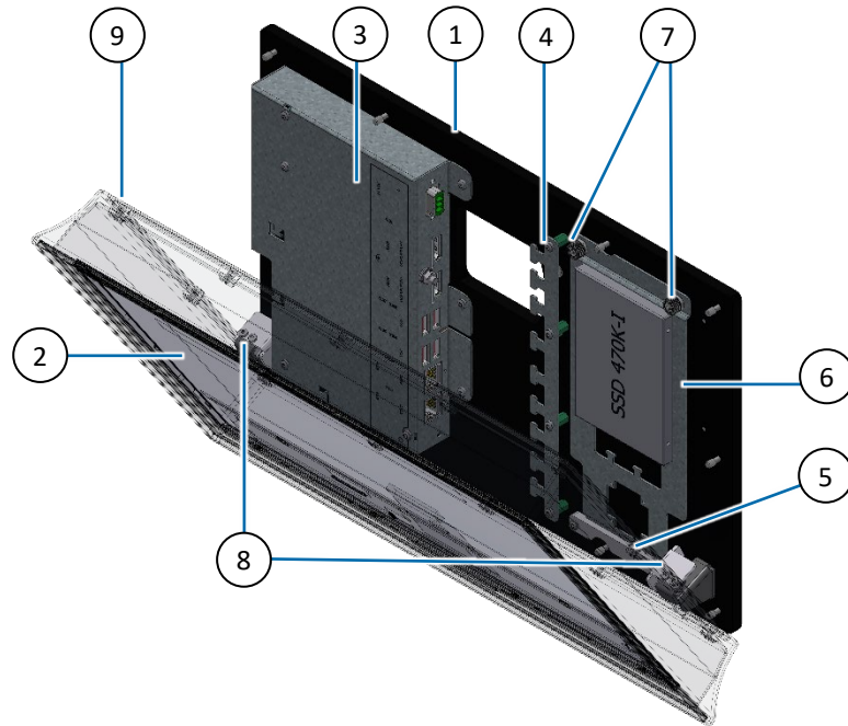
Figure 26: Accessing Internal Components for Maintenance
