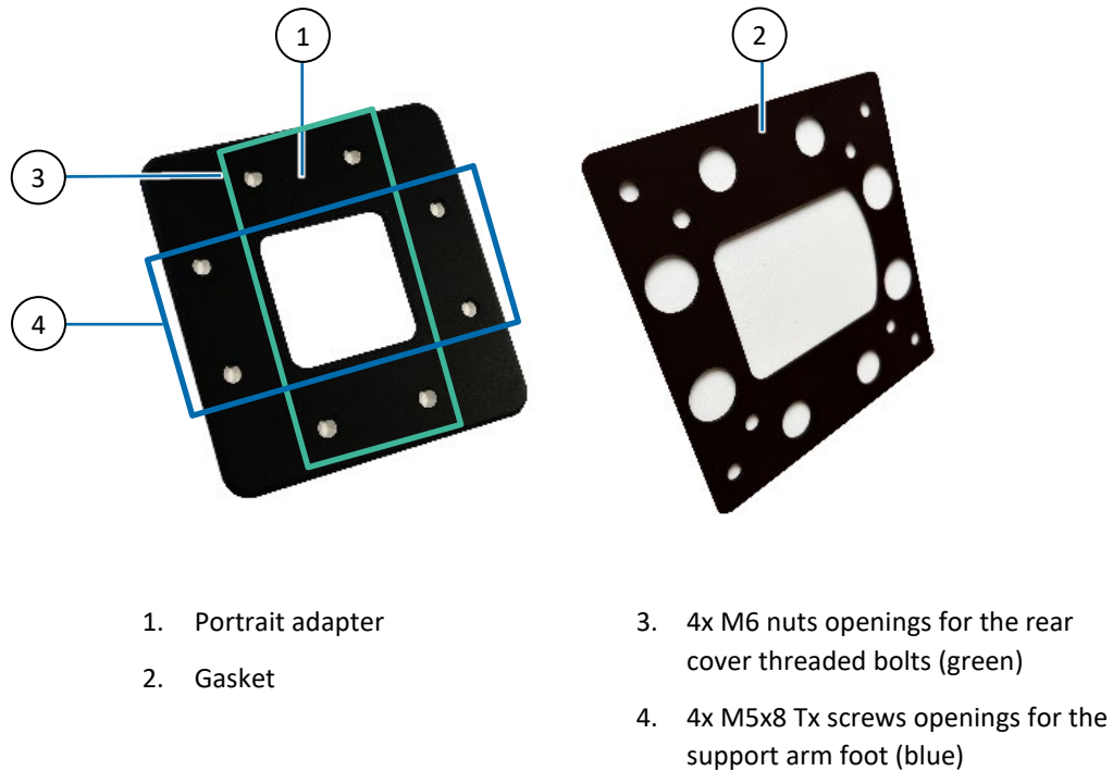
Figure 15: Portrait Adapter and Gasket
