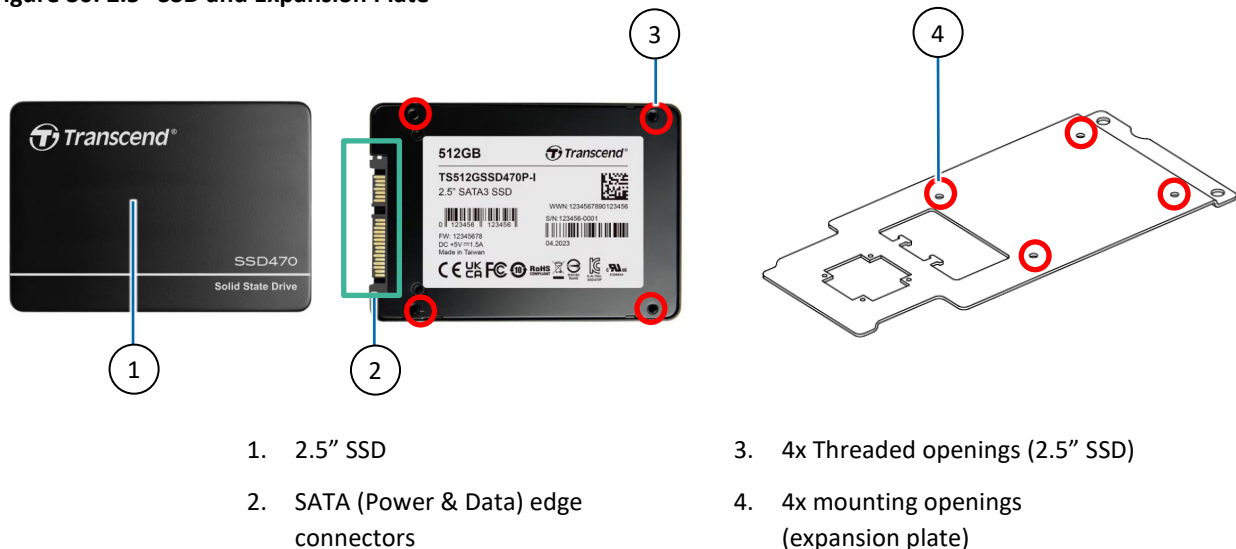
Figure 30: 2.5" SSD and Expansion Plate
