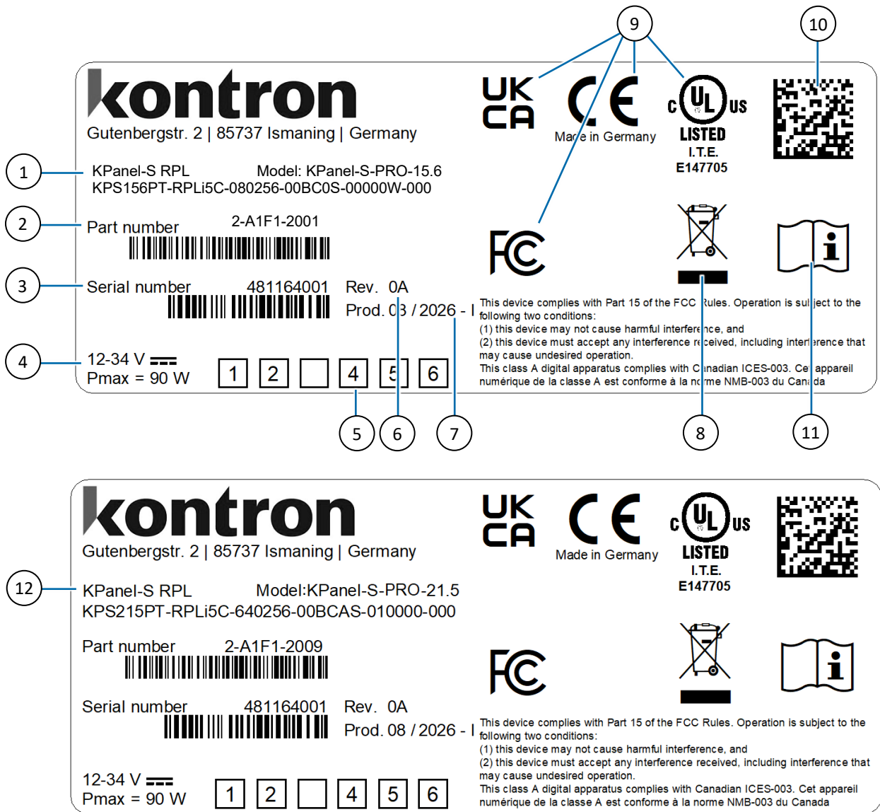
Figure 2: Type Label Examples (KPanel S-RPL-15.6 & KPanel S-RPL-21.5)
