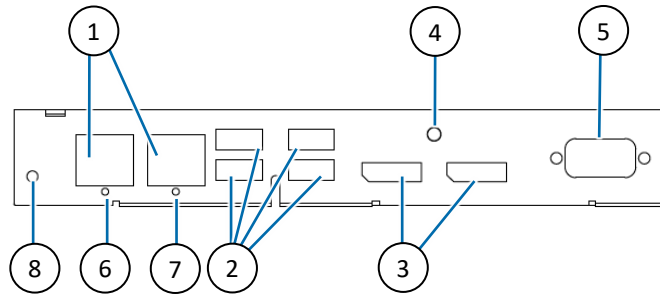
Figure 7: Interface Panel – KPanel S-RPL
