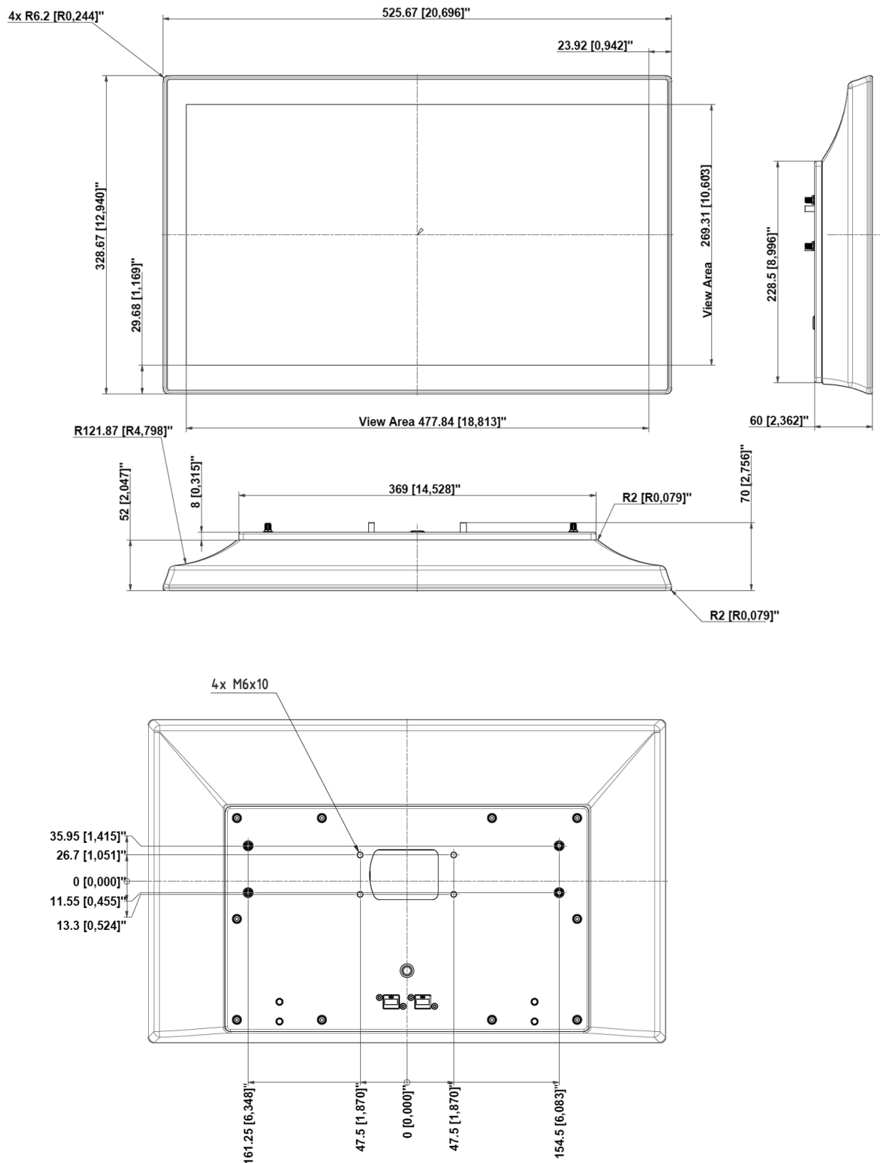
Figure 13: 21.5" Dimension Diagram (mm/inch)
