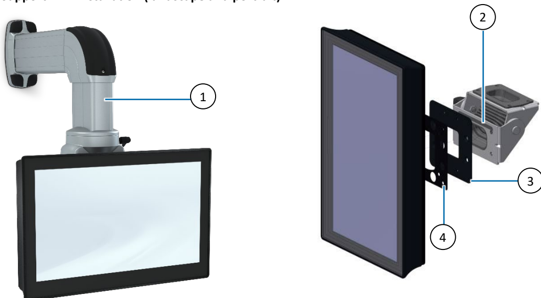
Figure 14: Support Arm Installation (landscape and portrait)
