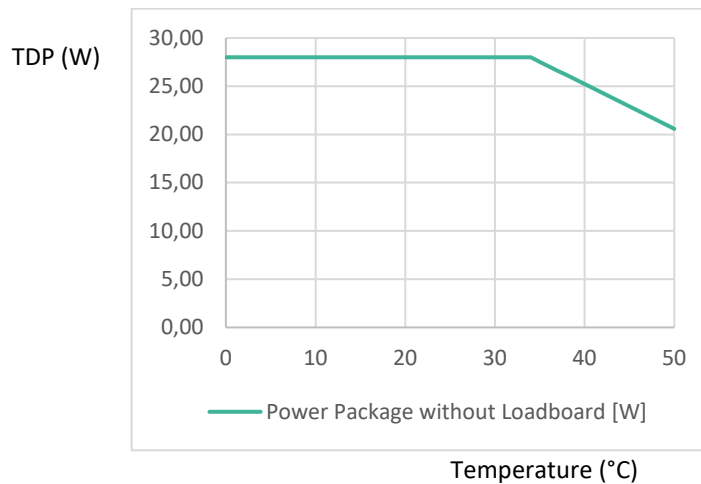
Figure 11: TDPs vs Temperature
