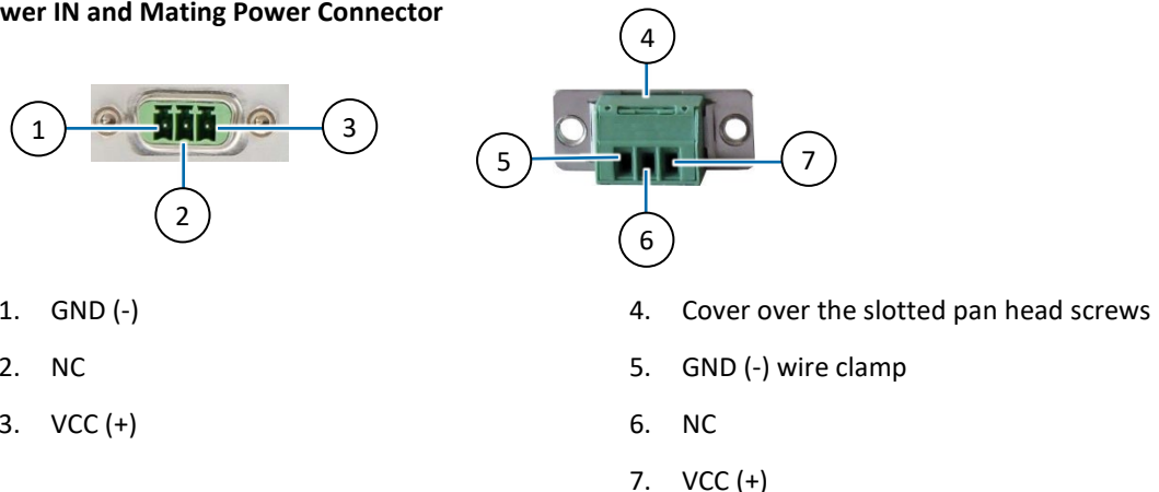
Figure 19: Power IN and Mating Power Connector
