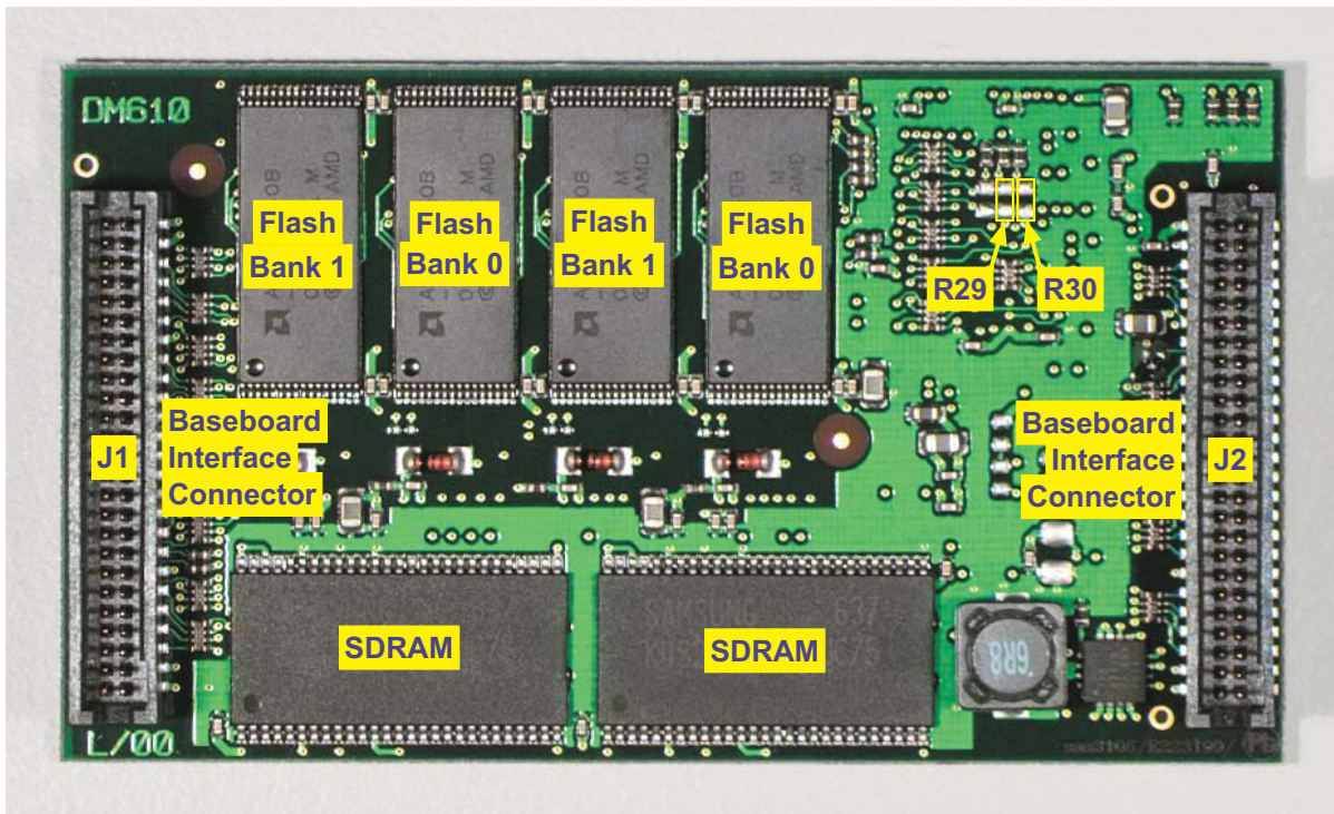
Figure 7-2: DM610 Board Layout (Bottom View)
