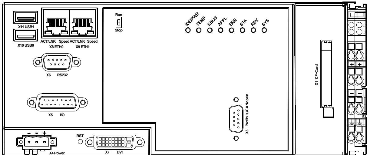
Figure 1-1: ThinkIO-Duo with PROFIBUS DP Fieldbus Option
