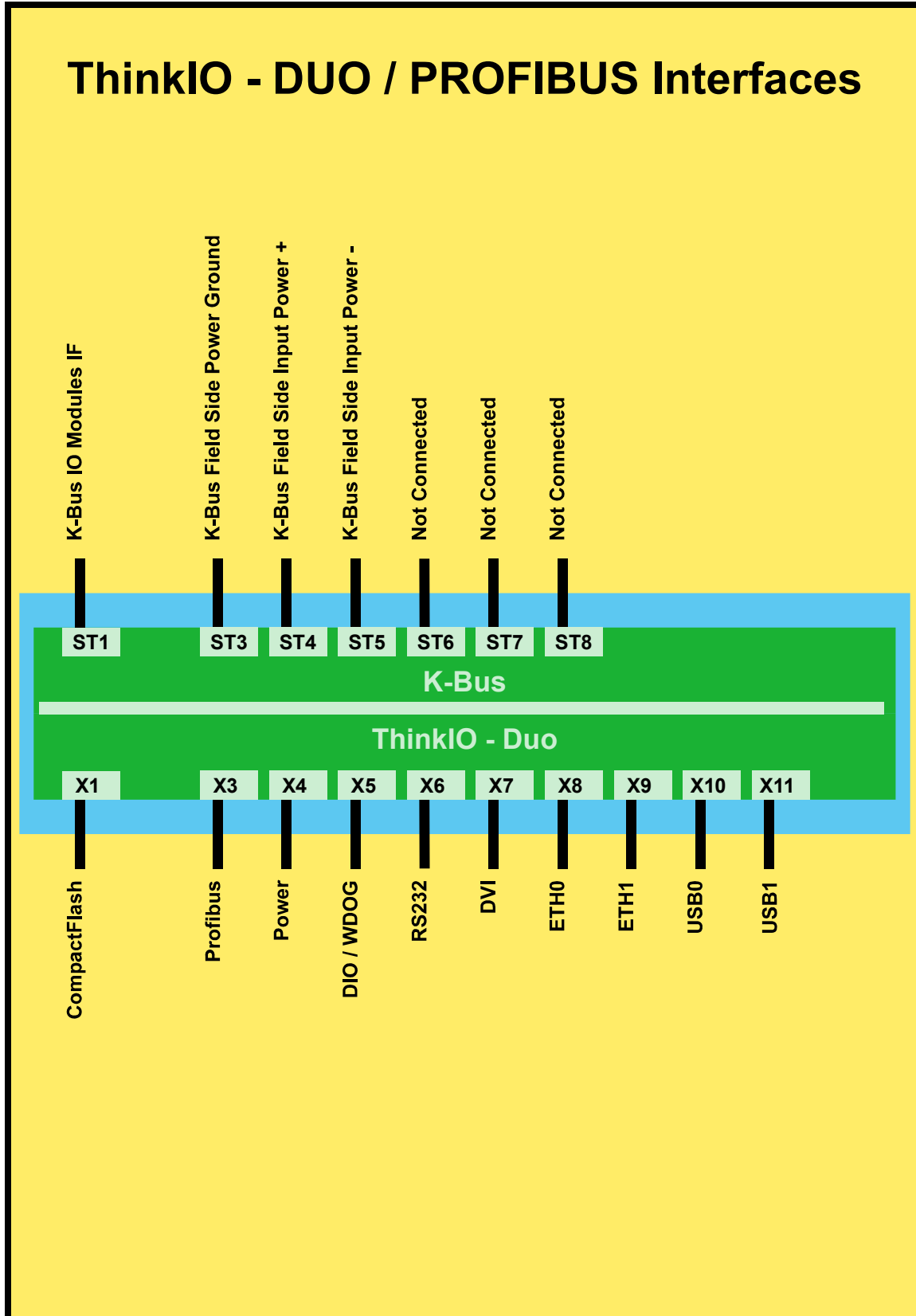
Figure 1-2: ThinkIO-Duo with PROFIBUS DP Fieldbus Option Interfaces
