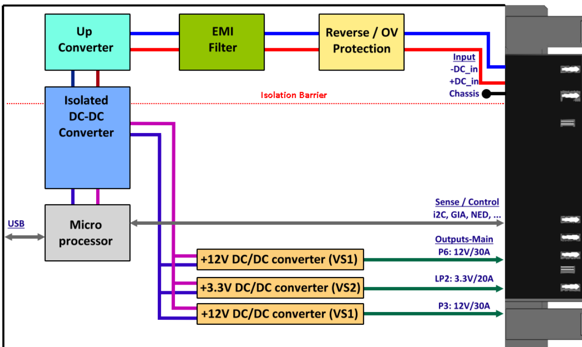
Figure 1: VPX-360DMS Block-Diagram
