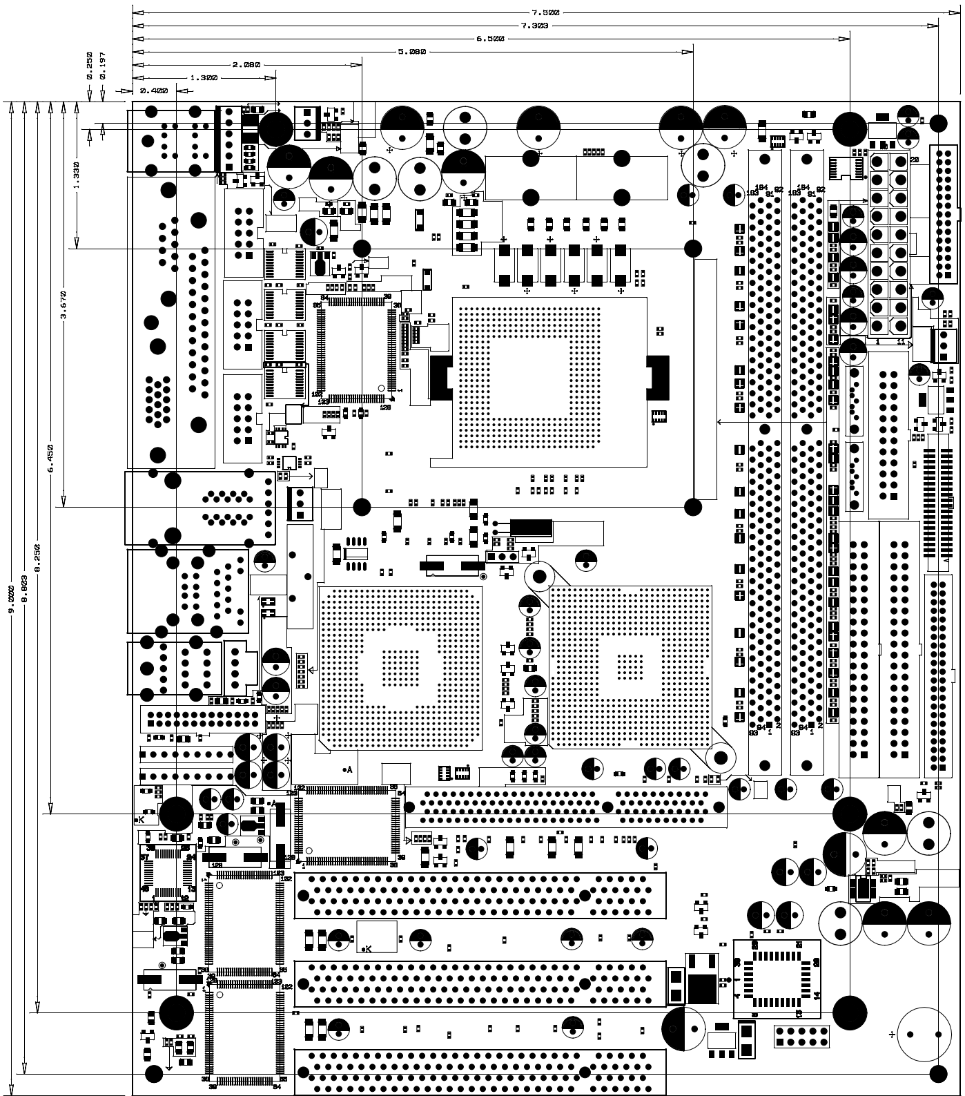
SILKSCREEN.TOP
