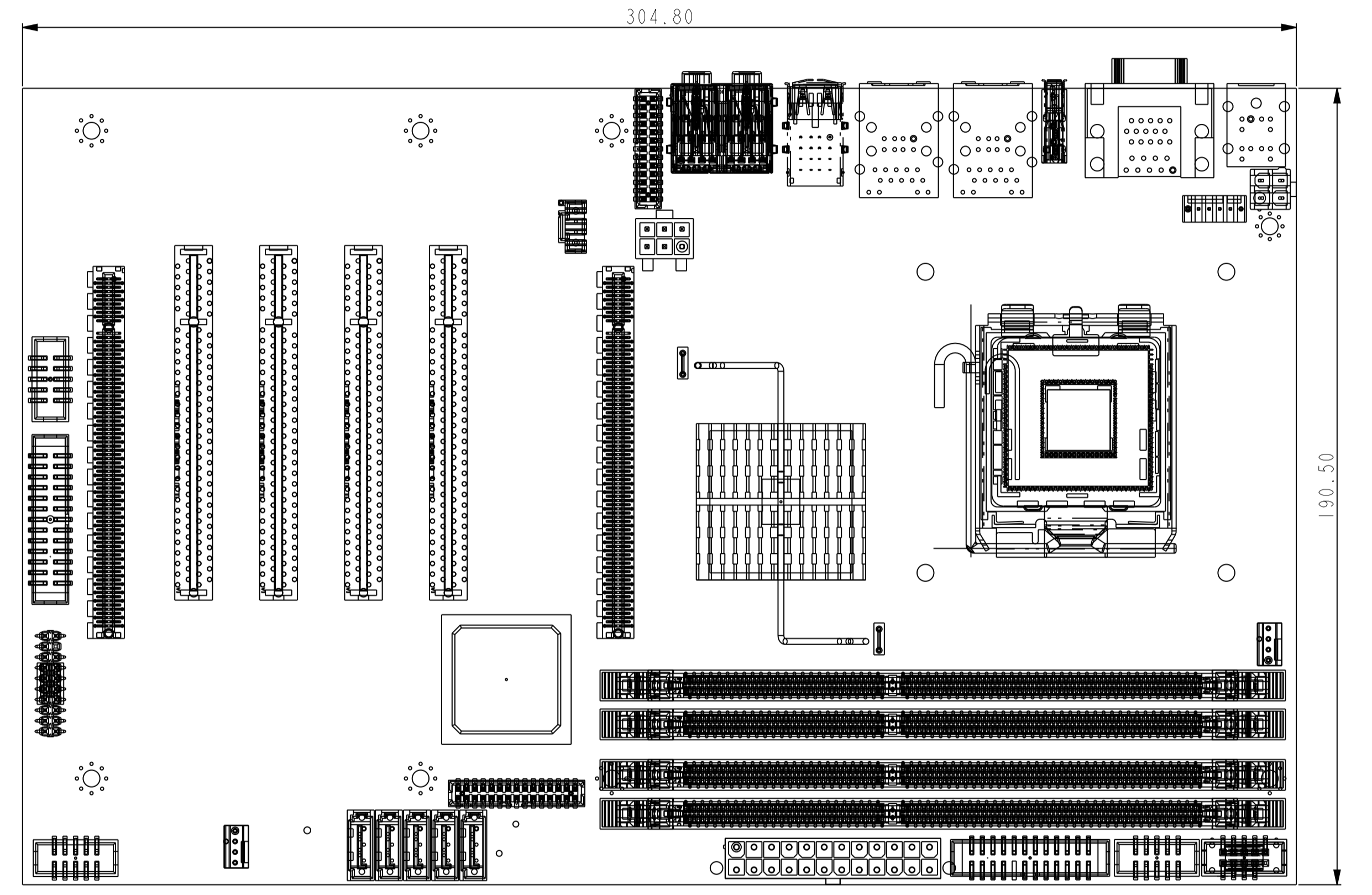
BOTTOM VIEW
