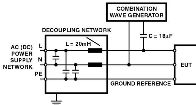
TEST SETUP FOR CAPACITIVE COUPLING ON AC/DC LINES; LINE TO LINE COUPLING ACCORDING TO 7.2
