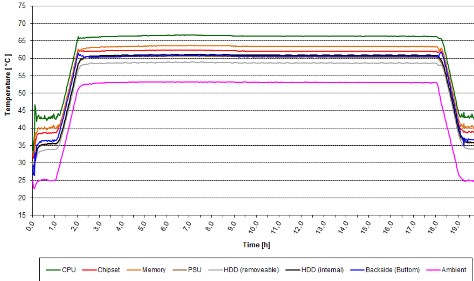
Fig. 5 Measurement diagram: High temperature, operating
