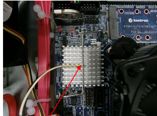
Chipset Sensor 2
