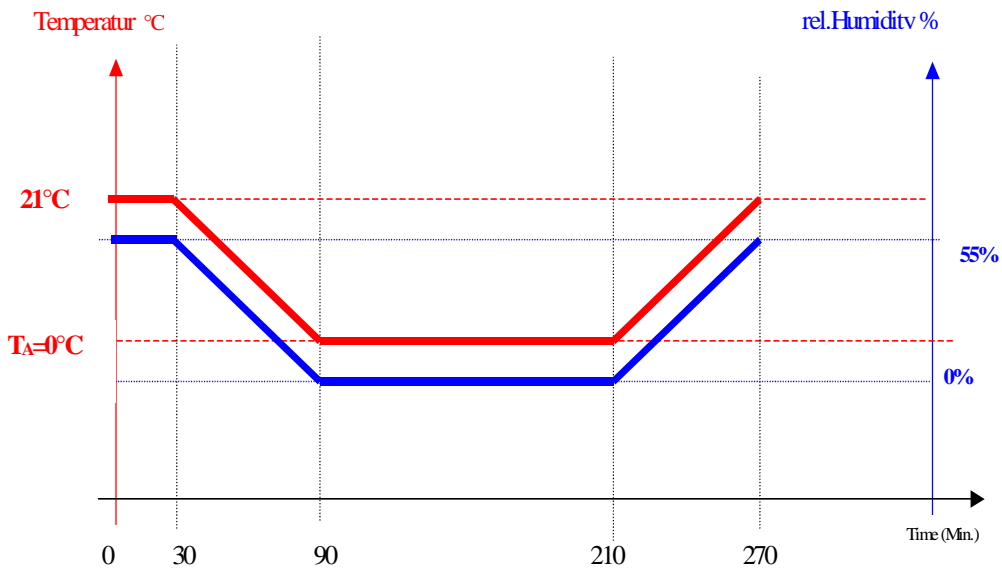
IEC 60068 PT2-30, Test Db: 12+12 Hour Cycle
