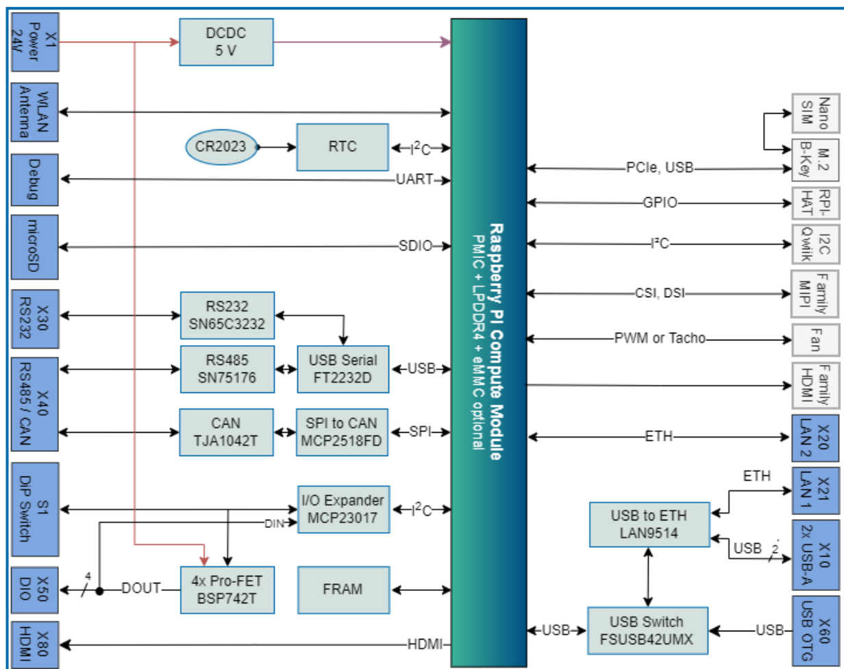
Figure 6: Block Diagram
