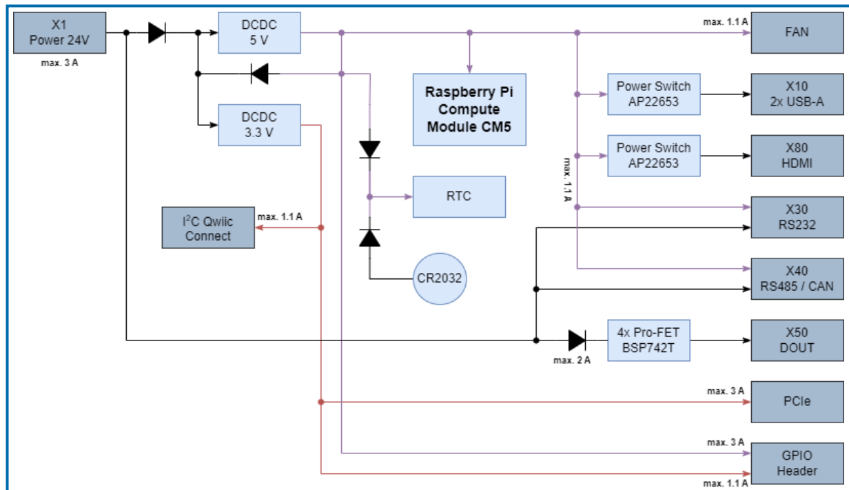
Figure 5: Power Tree
