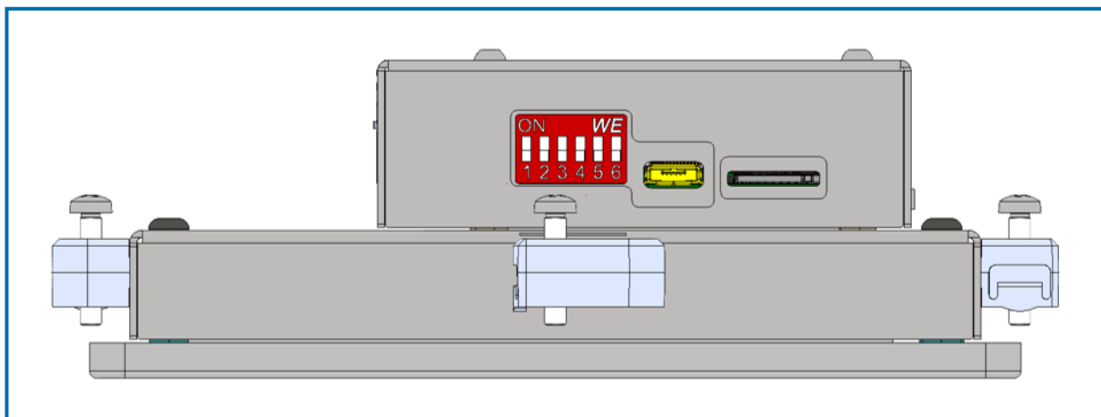
Figure 7: Side view right
