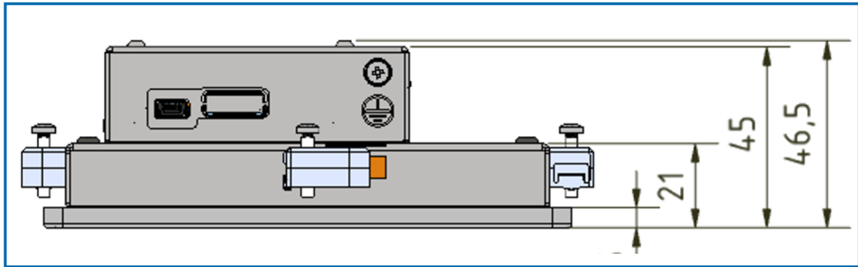
Figure 6: Side view left
