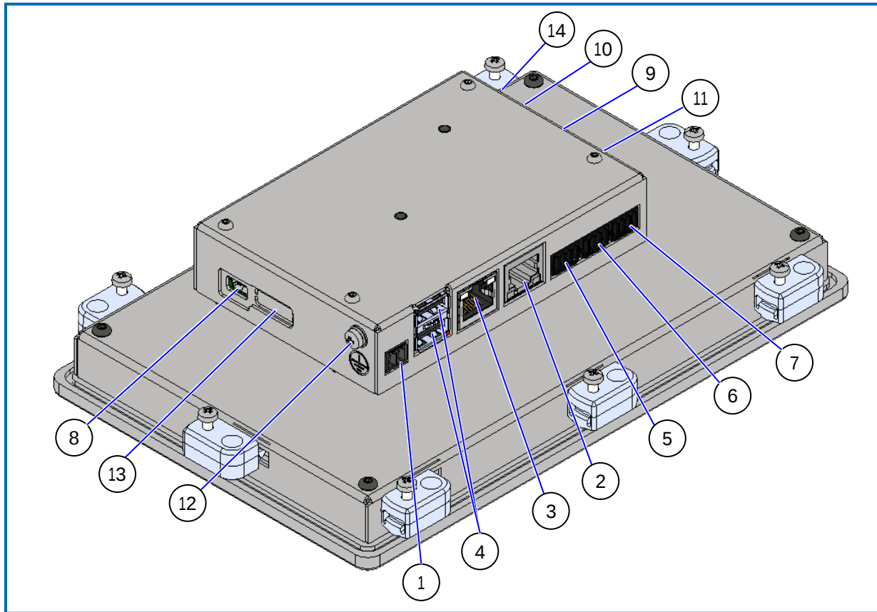
Figure 10: Top Side View
