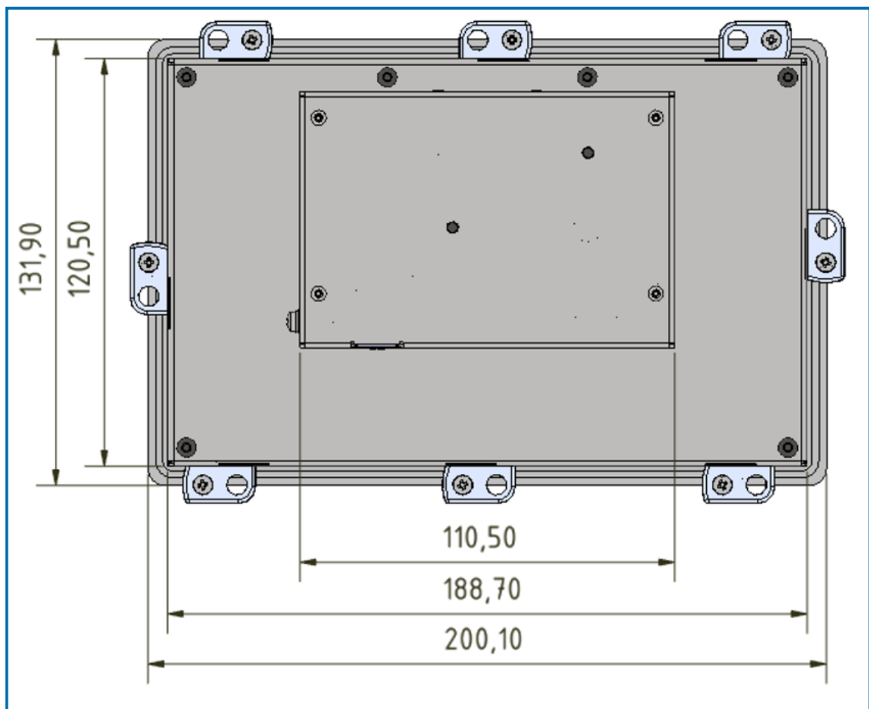
Figure 5: Rear View
