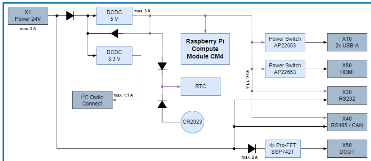
Figure 8: Power Tree
