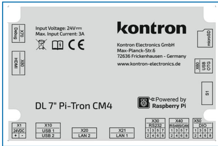
Figure 1: DL 7" Pi-Tron CM4 Type Label
